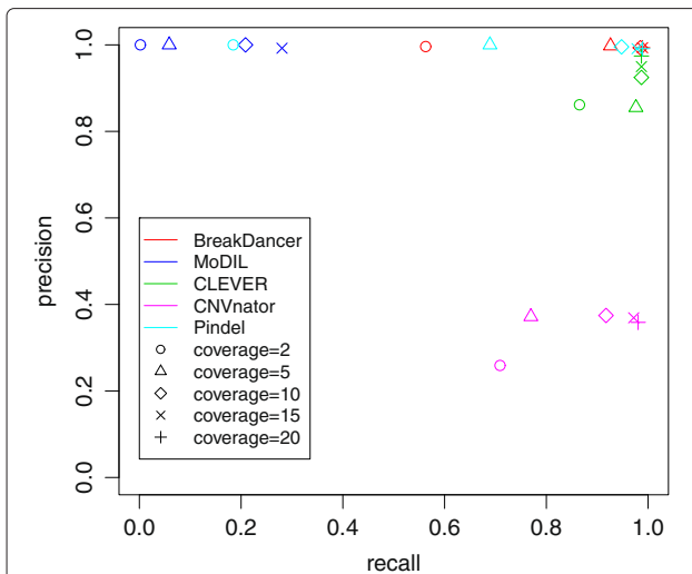
Figure 4 Recall and precision of results of SV detection tools. BreakDancer and CLEVER achieved relatively good recall for all coverage, while recall of MoDIL was low. Although recall of CNVnator was not bad, its precision was low. The recall of an SR method Pindel was good when coverage was high, but it was insufficient when coverage was low.
