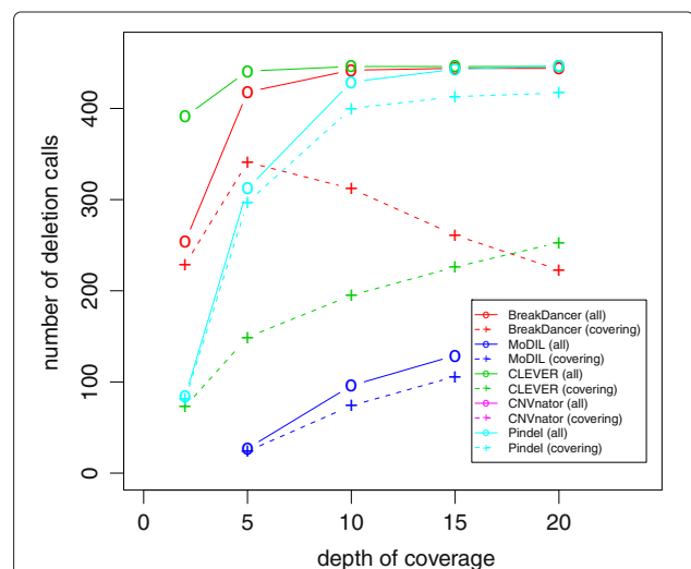
Figure 5 Number of deletion calls covering the whole of true deletions. Solid lines and circles show the number of all deletion calls generated by each tool, whereas dashed lines and '+' symbol show the number of deletion calls covering the whole of true deletions. Most of the deletion calls of MoDIL, CNVnator (expanded by the window size), and Pindel covered the whole of true deletions. On the other hand, many CLEVER results did not always contain the whole of true deletions, while median of the distribution of predicted breakpoints was close to the true breakpoints as shown in Figure 10. BreakDancer results for high coverage data did not always contain true deletions either. Predicted breakpoints of BreakDancer approached true breakpoints as the depth of coverage increases, and sometimes intruded into true deletions when coverage was high.
