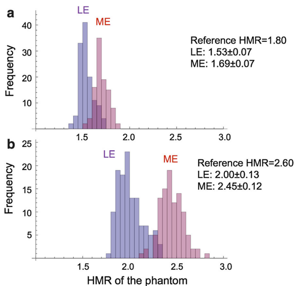
Figure 2. Distribution histograms of HMRs using phantoms with the reference HMR of 1.80 (a) and 2.60 (b). While the ME group shows higher values than the LE group, overlaps are observed.
