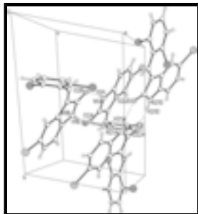
Fig. 2. : A unit cell packing view of the title compound. Dash lines indicate hydrogen bonds. For clarity, H atoms are presented as open circles with arbitrary radii.
