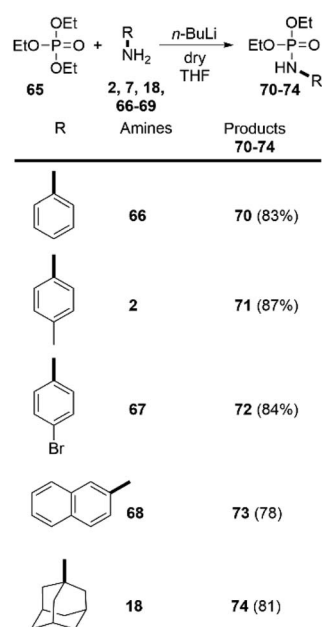
Scheme 5 Synthesis of phosphoramidates by direct amidation of triethylphosphate. Reaction conditions: 1.0 eq. of the corresponding amine and 2.0 eq. triethylphosphate; THF as solvent, and n -BuLi (2.0 eq.) as a base (at r.t. in inert atmosphere). Reaction time 5 min.
