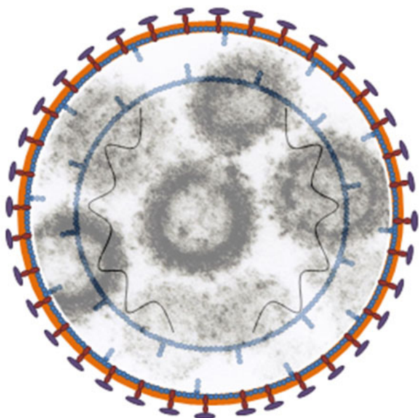
Figure 1 The cartoon of the L-2 particle has 7–10 times more envelope spikes compared to HIV and shows the double membrane of immature gag. Inside the picture is a TEM image of L-2 particles.
