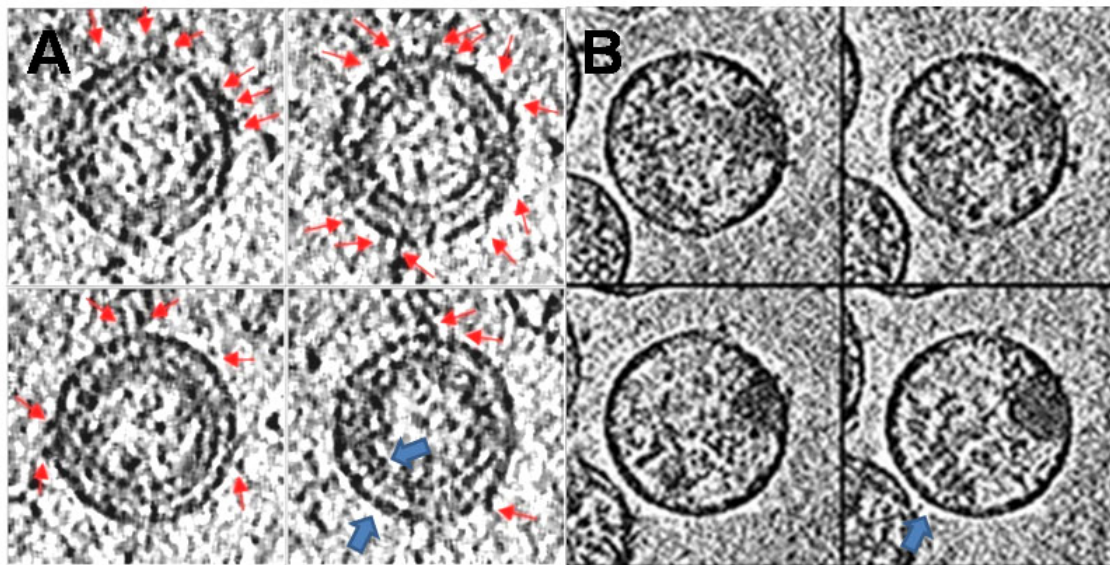
Figure 2 Cryo-EM images: A) The L-2 images show many envelope spikes (red arrows) and a double membrane (blue arrows). B) The control HIV shows few envelope spikes and a single membrane (blue arrow).
