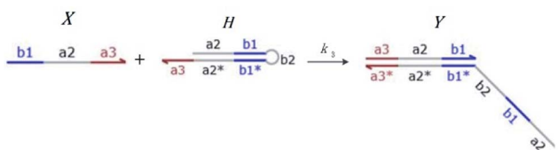
Fig. 2 DNA strand displacement with a hairpin structure. The toehold b_1 is as long as the other toeholds. The hairpin cannot open spontaneously as a result of the dissociation of b_1 - b_1^* hybridization at the end of the branch migration, the loop portion a_2 - b_1 - b_2 of the hairpin is protected if it does not open.
