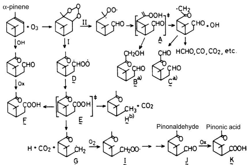
Figure 7.2.8 Reaction path of \alpha -pinene ozonolysis.
