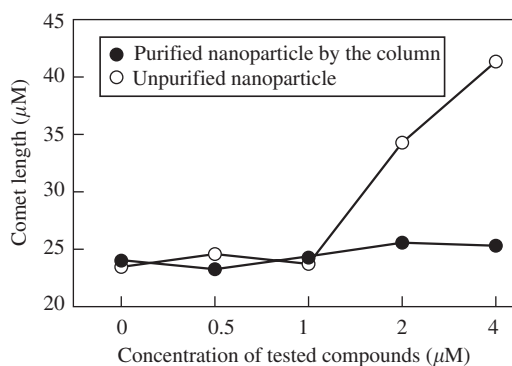
Figure 7.3.8 Cyto-toxicity of nanoparticles by the Comet Assay.
