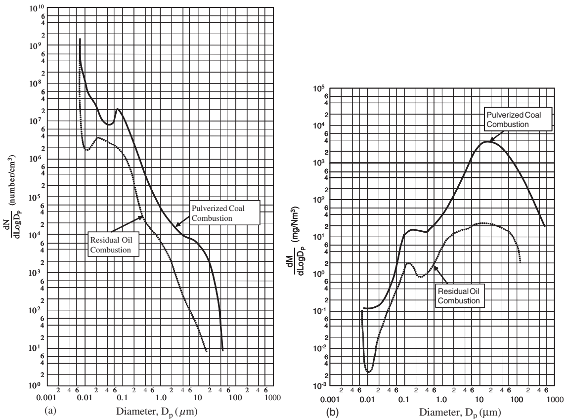
Figure 7.2.5 (a) Particle size distribution on number basis at combustor outlet. (b) Particle size distribution on mass basis at combustor outlet.
