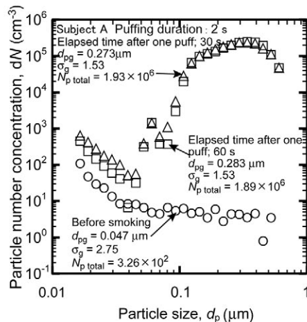
(b) Change in particle size distribution with the elapsed time after one puff of smoke by subject A
