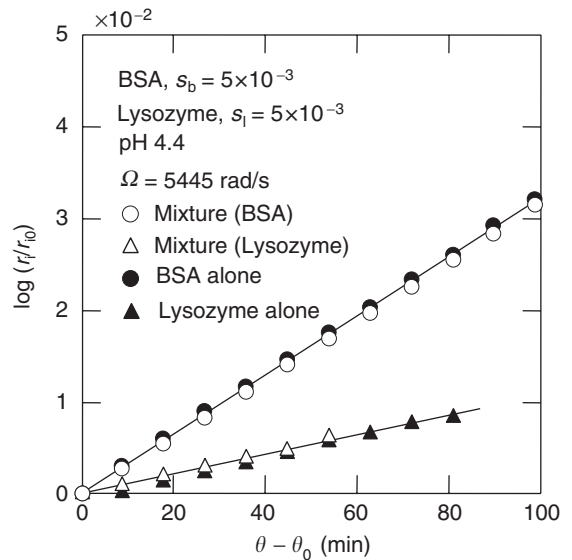
Figure 7.4.12 Behaviors of ultracentrifugal sedimentation of binary protein mixtures at pH 4.4.
