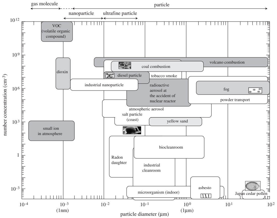
Figure 7.2.1 Particle size and concentration of various aerosols.
