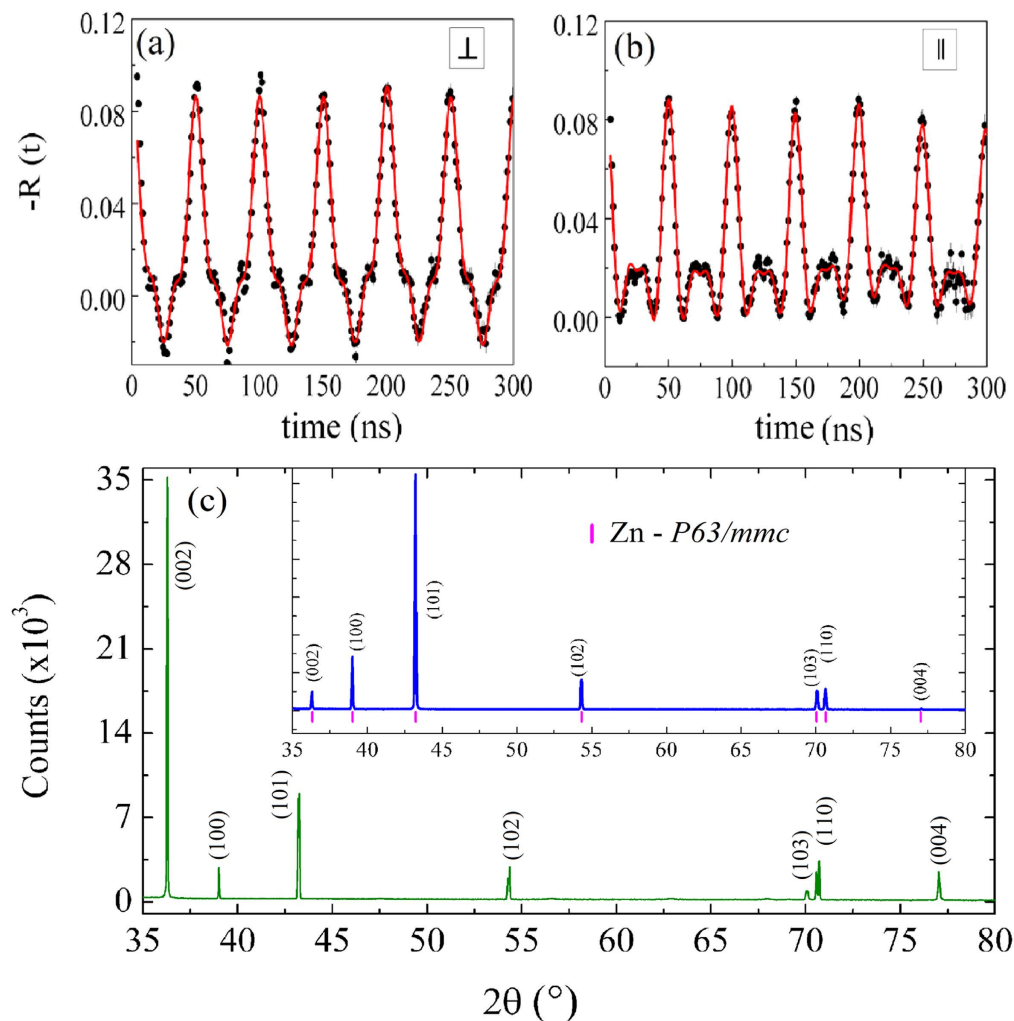
Figure 6. R(t) spectra at room temperature for: (a) perpendicular and (b) parallel configuration relative to the plane of detectors for a hollow microtube obtained at 800°C for 5 hours. (c) XRD pattern of the oxidized Zn microwire for 30 min at 515°C revealing preferred orientation of (002) plane of the metallic phase. The inset shows XRD of a pure isotropic polycrystalline metallic Zn microwire.
