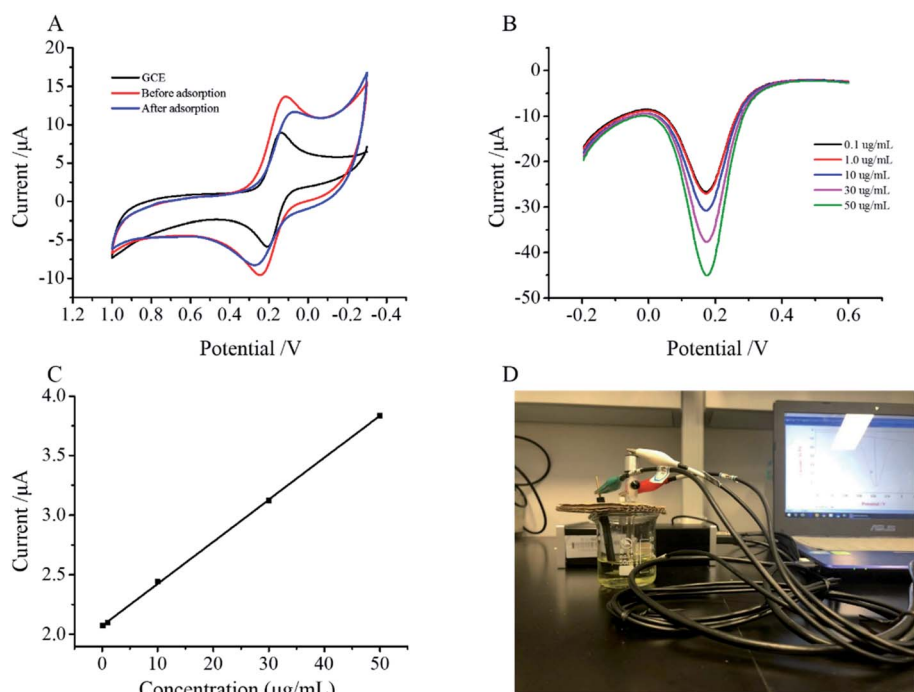
Fig. 6 (A) Cyclic voltammograms of different electrodes in the characterization solution, (B) differential pulse voltammograms of the different concentration aspartame standard solutions, (C) linear curve of aspartame standard solution, and (D) the portable electrochemical detection station.
