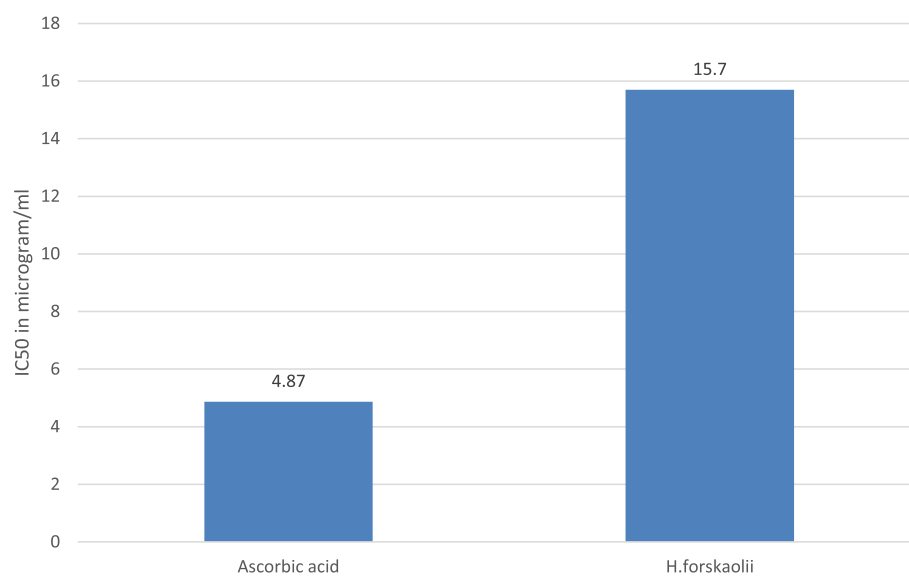
Figure 2 Experimentally determined IC 50 values of the leaf of H. forskoolii extract and ascorbic acid. Abbreviation: IC 50 , IC 50 values of the tested compounds in the concentration required to scavenge 50% of DPPH free radicals.
