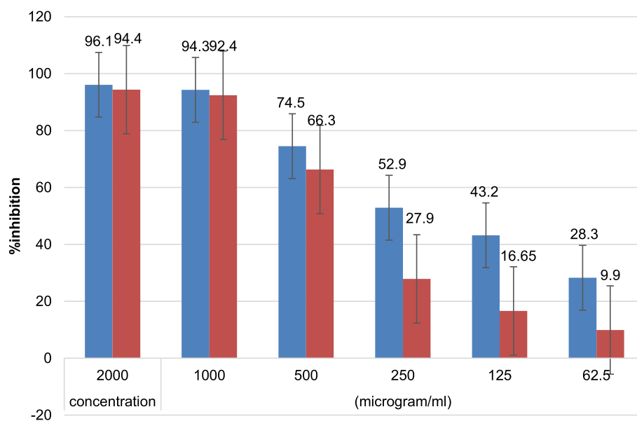
Figure 1 Free radical scavenging activity of the leaf extract of Hypoestes forskoolii . Abbreviations: SAA, scavenging percent of ascorbic acid; shef, scavenging percent for H. forskoolii .
