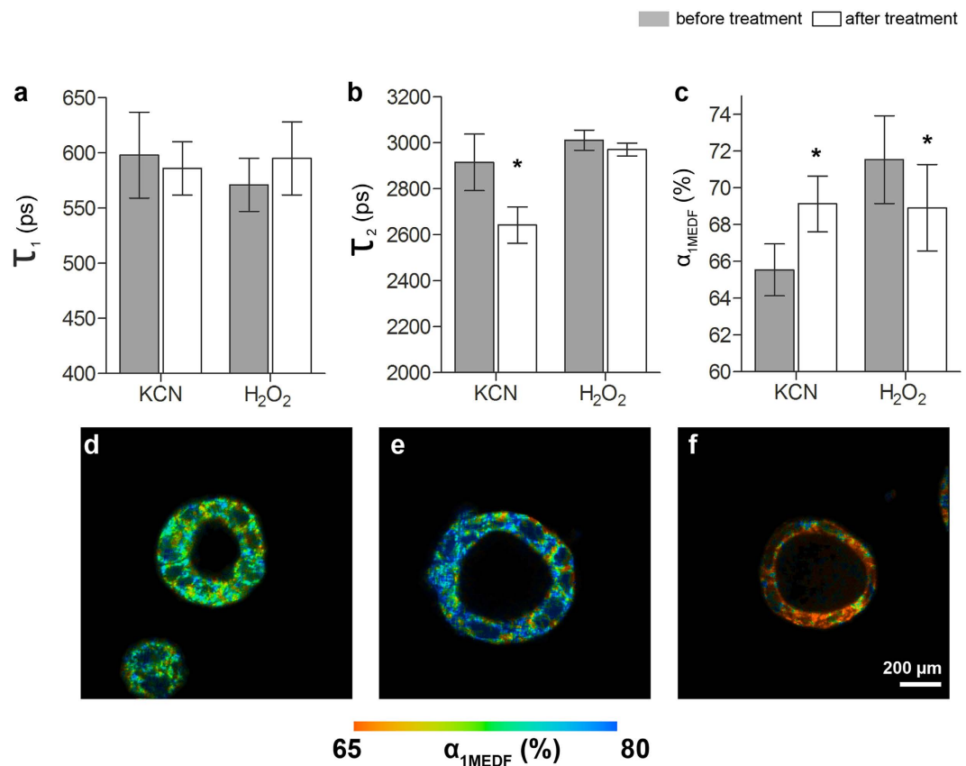
Figure 1. Multi-exponential decay fitting FLIM characteristics of 3D Caco-2 luminal cysts which are untreated and treated with KCN or H 2 O 2 . (a) \tau_1 of 3D Caco-2 luminal cysts before and after treatment with KCN (n = 6) or H 2 O 2 (n = 4). No significant impact is seen on the short fluorescence lifetime \tau_1 of NADH. (b) \tau_2 of 3D Caco-2 luminal cysts before and after treatment with KCN or H 2 O 2 . Treatment with KCN induces a significant decrease of \tau_2 (n = 6, *p = 0.0004), whereas no significant impact was detected on \tau_2 when treated with H 2 O 2 . (c) Changes are seen in the short fluorescence lifetime contribution \alpha_{1MEDF} before and after treating 3D Caco-2 luminal cysts with KCN or H 2 O 2 : Treatment with KCN induces an increase in \alpha_{1MEDF} (n = 6, *p = 0.0029), whereas H 2 O 2 treatment leads to a decrease in \alpha_{1MEDF} (n = 4, *p = 0.0434). (d–f) False color-coded images of (d) untreated, (e) KCN-treated, and (f) H 2 O 2 -treated 3D Caco-2 luminal cyst models indicating the range of \alpha_{1MEDF} from 65% (red) to 80% (blue).
