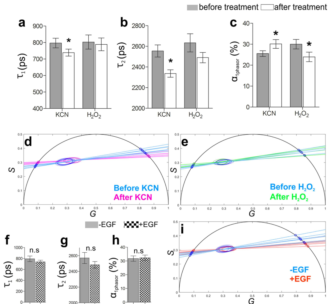
Figure 5. Phasor analysis of FLIM data from KCN-, H_2O_2 - and EGF-treated 3D Caco-2 models. (a) \tau_1 derived from phasor analysis before and after treatment with KCN ( n = 6 ) or H_2O_2 ( n = 4 ). KCN treatment induces a significant reduction in \tau_1 ( n = 6 , *p = 0.0007 ). (b) KCN treatment of 3D Caco-2 luminal cysts induces a significant decrease of \tau_2 ( n = 6 , *p = 0.0003 ). (c) 3D Caco-2 luminal cysts treated with KCN displayed a significant increase in the short fluorescence lifetime contribution \alpha_{1\text{phasor}} ( n = 6 , *p = 0.0169 ), whereas H_2O_2 leads to a decrease in \alpha_{1\text{phasor}} ( n = 4 , *p = 0.0113 ). (d) Phasor plot of 3D Caco-2 models before and after treatment with KCN shows 95% confidence ellipses and fitted linear functions on the universal circle. (e) Phasor plot of 3D Caco-2 models before and after H_2O_2 treatment reveals 95% confidence ellipses and fitted linear functions. (f–h) EGF treatment of 3D Caco-2 luminal cysts shows no significant changes in phasor analysis-derived (f) short fluorescence lifetime \tau_1 , (g) long fluorescence lifetime \tau_2 and (h) the short fluorescence lifetime contribution \alpha_{1\text{phasor}} of NADH ( n = 4 ). (i) Phasor plot of untreated and EGF-treated 3D Caco-2 models, showing 95% confidence ellipses and fitted linear functions on the universal circle. All phasor calculations were made with harmonic number k = 2 and usage of first half the period.
