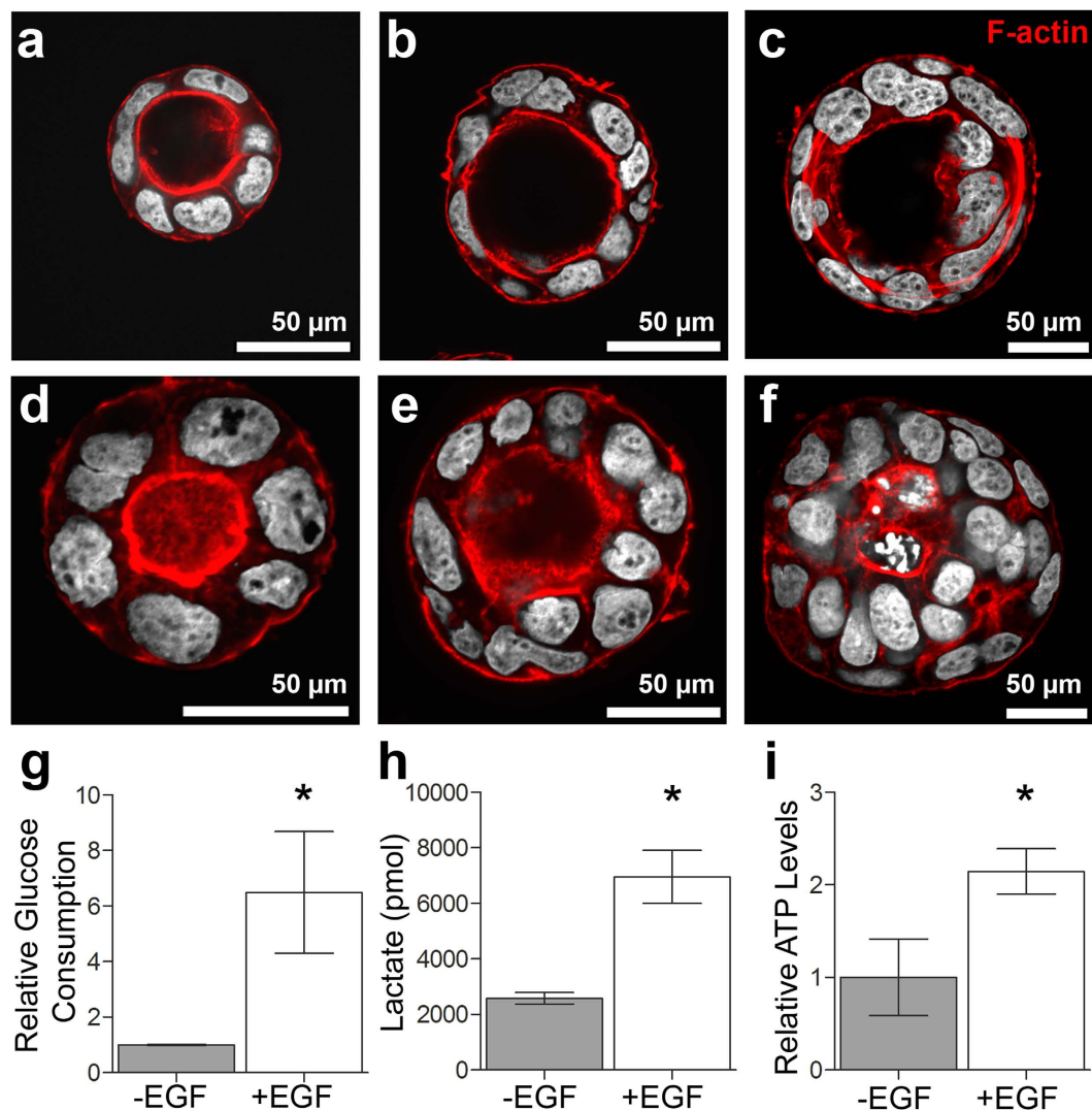
Figure 2. Morphology and metabolic behaviour of 3D Caco-2 luminal cysts treated with EGF. Fluorescence micrographs of 3D Caco-2 luminal cysts: (a–c) untreated and (d–f) treated with EGF. F-actin is shown in red and nuclei are depicted in white. (g) EGF treatment lead to a significant increase in relative glucose consumption ( n = 4 , *p = 0.0024 ). (h) Lactate production levels in EGF-treated 3D Caco-2 luminal cysts were significantly increased ( n = 4 , *p = 0.0001 ). (i) A significantly higher content of ATP is seen in EGF-treated 3D Caco-2 luminal cysts ( n = 4 , *p = 0.0031 ).
