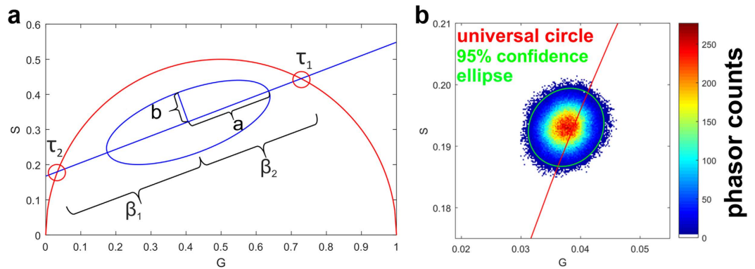
Figure 4. Explanation and validation of phasor plot approach. (a) Schematic of phasor plot properties showing the intersections of linear fitted line with universal circle representing lifetimes (e.g. \tau_1 and \tau_2 ) of contributing fluorophores for bi-exponential decays. Lifetime contributions \beta_1 and \beta_2 show distance of mean of phasor data from \tau_1 and \tau_2 . Shape of the phasor data is determined with calculation of 95% confidence ellipse. Relative lifetime contribution \alpha_i ( i = 1, 2 ) is calculated using \alpha_i = \beta_i / (\beta_1 + \beta_2) . Elliptical ratio a/b , determined by semi-major axis a and semi-minor axis b gives further information about fluorescence properties. (b) Phasor plot of FLIM signal from coumarin 6. Green ellipse represents the 95% error ellipse of phasor approach calculations. Ratio between major and minor semi-axis is a/b = 1.13 and the subsequent fluorescence lifetime is \tau_{\text{coumarin}} = 2.48 ns. Calculations were made with harmonic number k = 4 and usage of first quarter of period.
