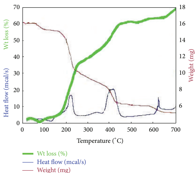
FIGURE 3: TGA and DSC curves for \text{Cs}_x\text{H}_{3-x}\text{PW}_{12}\text{O}_{40}/\text{Fe-SiO}_2 precursor.
