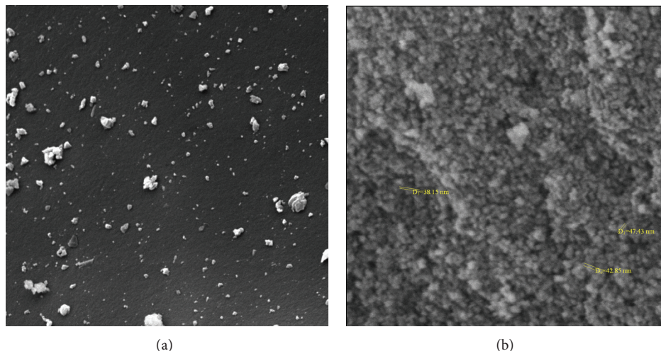
FIGURE 4: The SEM images of Cs_xH_{3-x}PW_{12}O_{40}/Fe-SiO_2 nanocatalyst, (a) precursor and (b) calcined catalyst.
