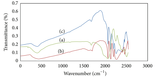
FIGURE 1: FT-IR spectra of the Cs_XH_{3-X}PW_{12}O_{40}/Fe-SiO_2 (a), H_3PW_{12}O_{40} (b), and Cs_XH_{3-X}PW_{12}O_{40} (c) nanocatalysts.
