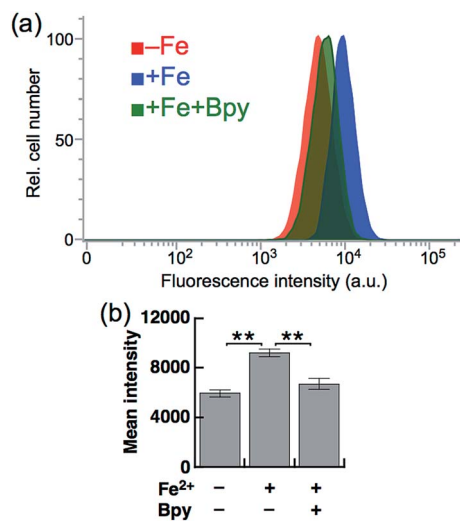
Fig. 4 (a) Representative flow cytometry histograms of control cells treated with 5 \mu M SiRhoNox-1 for 1 h (red), cells treated with 100 \mu M Fe 2+ (FAS) for 30 min prior to staining with 5 \mu M SiRhoNox-1 for 1 h (blue), and cells treated with 100 \mu M Fe 2+ (FAS) for 30 min prior to staining with 5 \mu M SiRhoNox-1 in the presence of 1 mM Bpy for 1 h (green). A total of 10 000 cells was analyzed for each histogram. (b) Mean intensities of fluorescence observed by flow cytometry. Statistical analyses were performed with a Student's t -test. ^{***}P < 0.01 ( n = 5 ). Error bars indicate \pm S.E.M.
