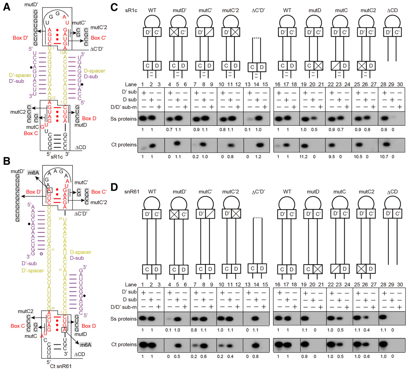
Figure 4. Box C/D and C'/D' are functionally independent. (A, B) Secondary structure of archaeal sR1c (A) and eukaryotic Ct snR61 (B) RNAs. The analyzed mutations (mut) and deletions ( \Delta ) are illustrated. The locations of m 6 A modification in box D and D' of snR61 are marked. (C, D) Modification activity of C/D RNPs assembled with sR1c (C) and snR61 (D) mutant RNAs. Ct RNPs were assembled with either C/D RNA (2 \mu M), Snu13 (6 \mu M), Nop56/Fib (2 \mu M) and Nop58/Fib (2 \mu M). Ss RNPs were assembled with either C/D RNA (1 \mu M), co-purified Nop5/Fib complex (2 \mu M) and L7Ae (3 \mu M). The D and D' substrates and mixed pre-methylated substrates (sub-m) were reacted for 20 min by Ct RNPs at 50°C and by Ss RNPs at 70°C. The relative level of modification shown under each band was normalized to that guided by wild-type sR1c or snR61.
