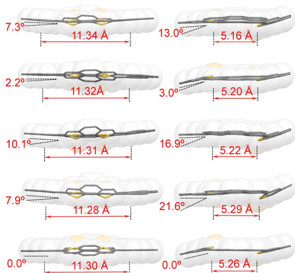
Fig. 3 Five kinds of different crystal structures of polymorphs of MS-4T , with the main view on the left and the corresponding side view on the right. All alkyl chains have been omitted.
