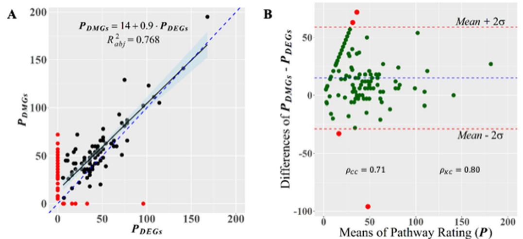
Figure 5. Graphical evaluation of the concordance between DEG and DMG enrichments on KEGG pathways. (A) scatterplot of pathway ratings (see Eq. 1) from enriched pathways on the set of DMGs ( P_{DMGs} ) and DEGs ( P_{DEGs} ), respectively. Regression analysis shows the linear trend of the relationship P_{DEGs} > 0 versus P_{DMGs} > 0 (black dots). The identity dashed line (in blue) helps in gauging the degree of agreement between measurements 26 . Dots in red highlight pathways for which P_{DEGs} = 0 or P_{DMGs} = 0 . (B) Bland-Altman plot of the agreement, on targeting gene pathways, between responses from gene expression and methylation regulatory systems. The agreement between measurements can also be tested by values of the Lin's concordance correlation coefficient ( \rho_{CC} ) and Kendall coefficient of concordance ( \rho_{KC} ).
