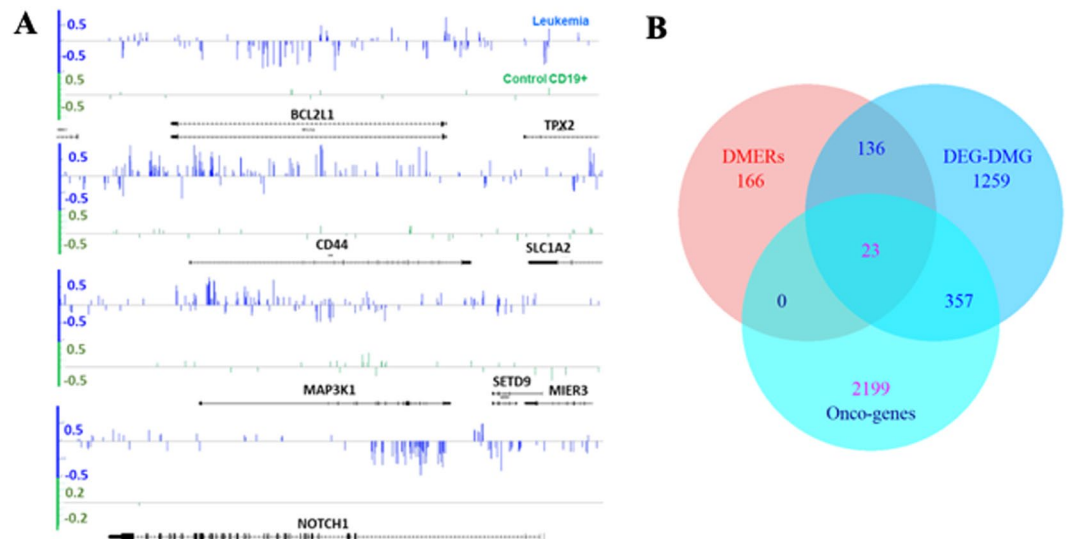
Figure 7. DEG-DMGs reported as cancer related gene lists. (A) Group mean of methylation level differences at each cytosine identified differentially methylated genes (DMGs). BCL2L1 , CD44 , MAP3K1 and NOTCH1 are linked to leukemia and other types of cancers. The genes were identified as PPI network hubs (Fig. 5B,D). Irregular distribution of methylation signal, hyper- and hypo- methylated, can be seen. Traditional DMR-based approaches fail to detect these types of variation. Methylation level differences were computed for control and treatment individuals with respect to normal CD19+ methylome from four independent blood donors used as reference. This approach provides an estimation of the natural variability of methylation changes existing in the control population. (B) Overlap ( \geq 500 bp) between differentially methylated enhancer regions (DMERs) and DEG-DMGs. Although only 51 enhancers (DMERs) are activators of reported DEGs, the DMERs overlap with 159 DEG-DMG regions, of which 23 are reported oncogenes (see Methods). A total of 379 DEG-DMGs are reported oncogenes.
