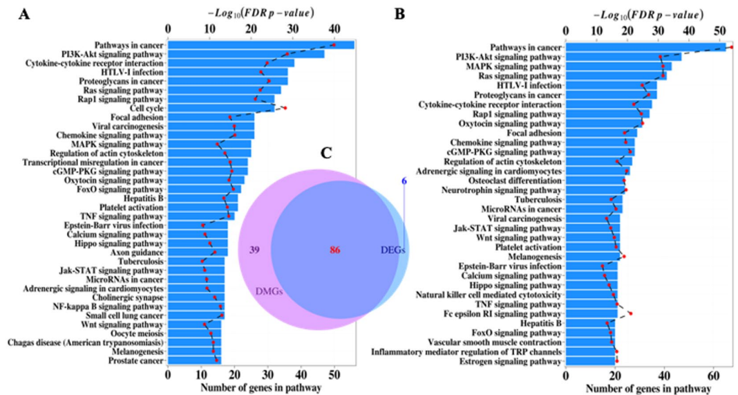
Figure 4. Network-based enrichment analysis of protein-protein interaction (PPI) networks independently derived from DMGs and DEGs estimated in patients with PALL. (A) PPI enriched network of DEGs with 15 or more genes. (B) PPI enriched network of DMGs with 20 or more genes. (C) Venn diagram with the overlapping of all PPI enriched networks of DMGs and DEGs with 7 or more genes. The PPI enriched network analysis was performed in STRING app on Cytoscape, 22,25 and the analysis is limited to KEGG human pathways.
