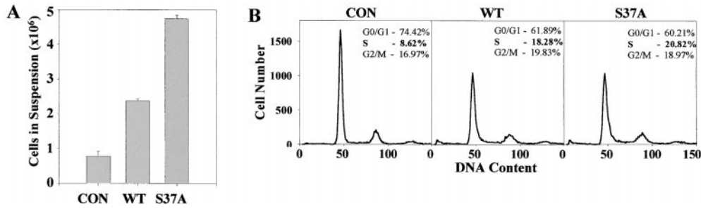
Figure 4. \beta -Catenin overexpression promotes proliferation at high cell density. A , Cells were cultured three days after confluence. After washing, cell shedding was measured over a 24 h period by counting the number of cells suspended in the medium. Graphing and SD calculation were performed using Sigmaplot. B , Cell cycle
