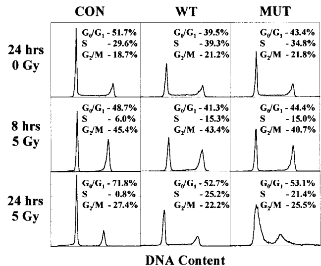
Figure 5. \beta -Catenin overexpression attenuates the \gamma -irradiation G 1 cell cycle block. Cells were \gamma -irradiated with 0 or 5 Gy. 8 and 24 h later, the cell cycle distribution was determined. The unirradiated cells all had a similar profile with the characteristic differences in G 0 /G 1 and S phases (see Fig. 3). The S phase population of CON cells is significantly reduced at 8 h and absent at 24 h. At 24 h, the CON cells were blocked entirely in the G 0 /G 1 or G 2 phases of the cell cycle. A slight decline in the proportion of WT and S37A cells in S phase occurs at 8 h after irradiation, but this is much less than that which occurs in CON cells. In contrast to CON cells, at 24 h the S phase proportions of the WT and S37A cells have partially recovered. All experiments were performed at least three times with consistent and repeatable results.
