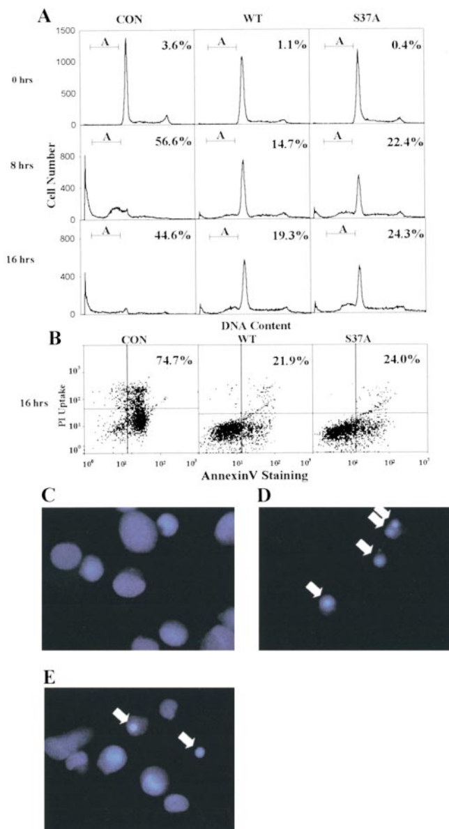
Figure 8. \beta -Catenin expression prevents anoikis. A , DNA/flow cytometric analysis of CON, WT, and S37A cells after incubation in suspension for 0, 8, or 16 h. The hypodiploid population corresponds to the apoptotic cells. The percentage in each panel represents the hypodiploid fraction. B , AnnexinV and propidium iodide staining of the same cells at 16 h also demonstrates a significant protection by \beta -catenin. C , Hoechst staining demonstrates nuclear morphology of CON cells before suspension. All nuclei look normal. WT and S37A cells looked similar. D , Hoechst staining of CON cells after 16 h in suspension. Most nuclei have a shrunken apoptotic morphology (arrows). E , S37A cells after 16 h in suspension. Most cells had the normal nuclear morphology, but a significant fraction ( \sim 25\% ) were shrunken apoptotic (arrows). Experiments represented in A and B were performed at least three times with consistent and repeatable results. Experiments represented in C–E were performed twice with consistent and repeatable results.
