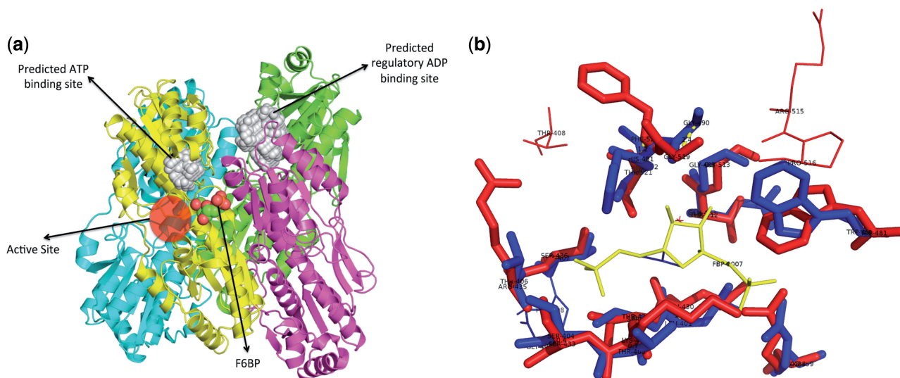
Figure 6. Examples for exploring protein–ligand interaction space. (a) Predicted binding sites in phosphofructokinase. Both the active site of the enzyme in its monomeric subunit along with regulatory binding site of ADP at the interface of subunits has been rightly picked up. (b) Superposition of the residues in the predicted binding site of PKM2 (pyruvate kinase) with the topmost hit of fructose-biphosphate (FBP) binding site. FBP is known to be an allosteric activator of PKM.
