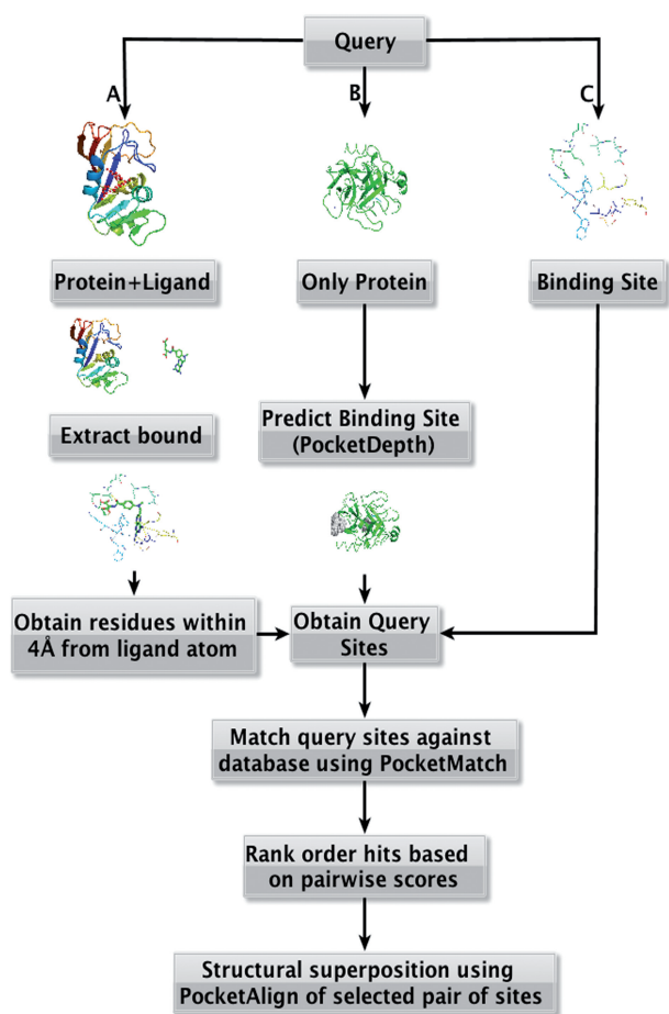
Figure 1. PocketAnnotate workflow. All the steps involved in the PocketAnnotate workflow for three different type of queries has been illustrated. (A) If a protein–ligand complex is chosen, the 4 Å region around the ligand is extracted and considered to be binding site. This extracted binding site is then compared against the database using PocketMatch, and the highest scoring similar pockets can be visualized using PocketAlign. (B) If Only protein option is chosen, the pockets are predicted for the protein using PocketDepth. The suitable pocket can then be compared with pockets in the database using PocketMatch, and relevant hits can be subjected to PocketAlign to obtain the annotation for the pocket of interest. (C) Only substructure of a protein can also be given as input and can be compared against the database to obtain the similarity with other binding sites using PocketMatch and PocketAlign.
