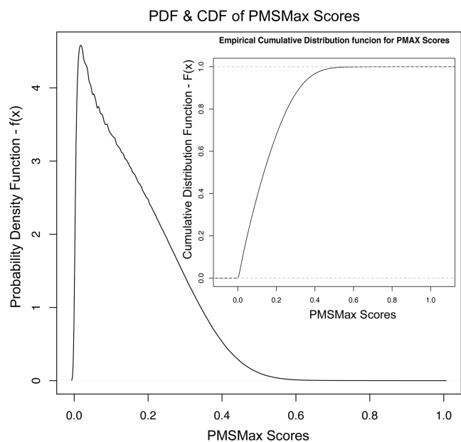
Figure 3. Distribution of PMS_{MAX} scores. Probability density function of the PMS_{MAX} distribution of all versus all pairwise comparisons in the data set. Starting from a frequency histogram of PMS scores in data set comparison, the probability density graph is obtained by using a kernel density estimation method with smoothing parameter (bandwidth) of 0.002311. The inset shows the cumulative distribution for the same data. (Refer text for mathematical description).
