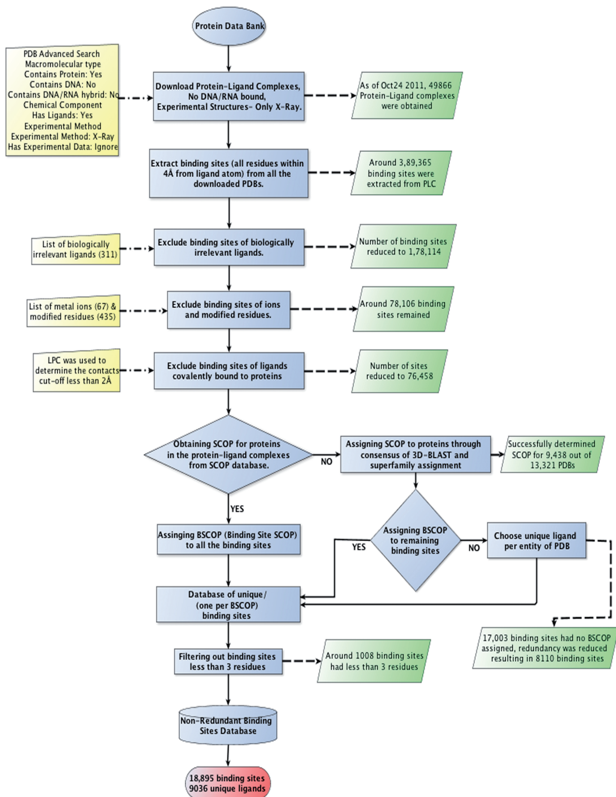
Figure 2. Non-redundant binding site database. All the steps involved in generation of non-redundant binding sites based on SCOP association has been illustrated.
