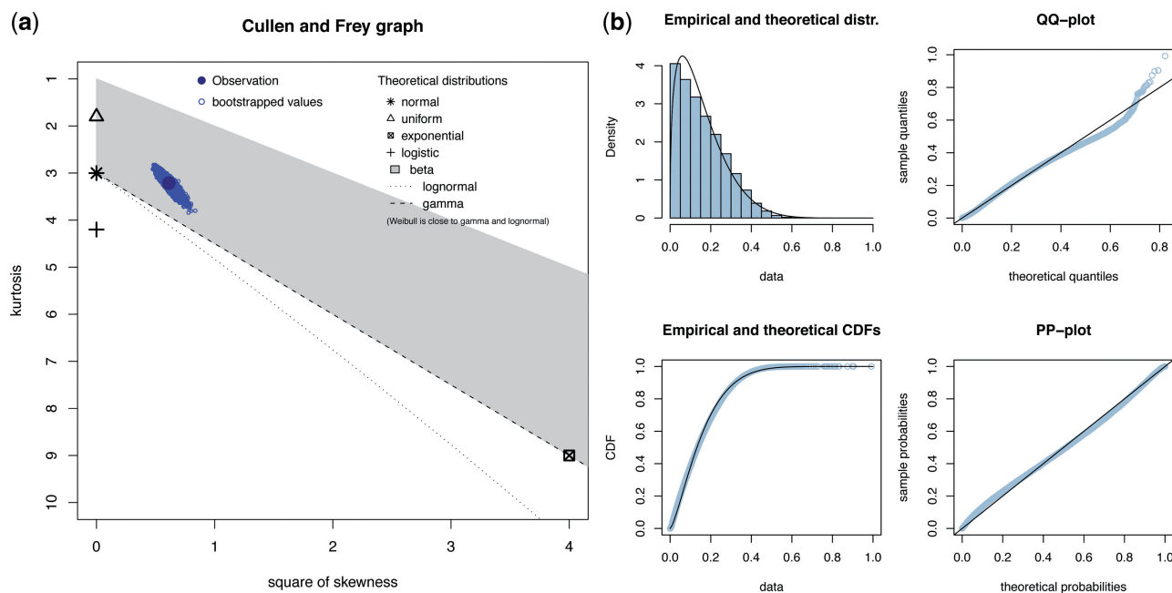
Figure 4. Statistical analysis and distribution fitting of all versus all PMS_{MAX} scores from pocket comparisons in the data set. (a) Cullen and Frey analysis suggesting that data points observed follows beta distribution. [b(i-iv)] Goodness of fit to the estimated beta distribution.
