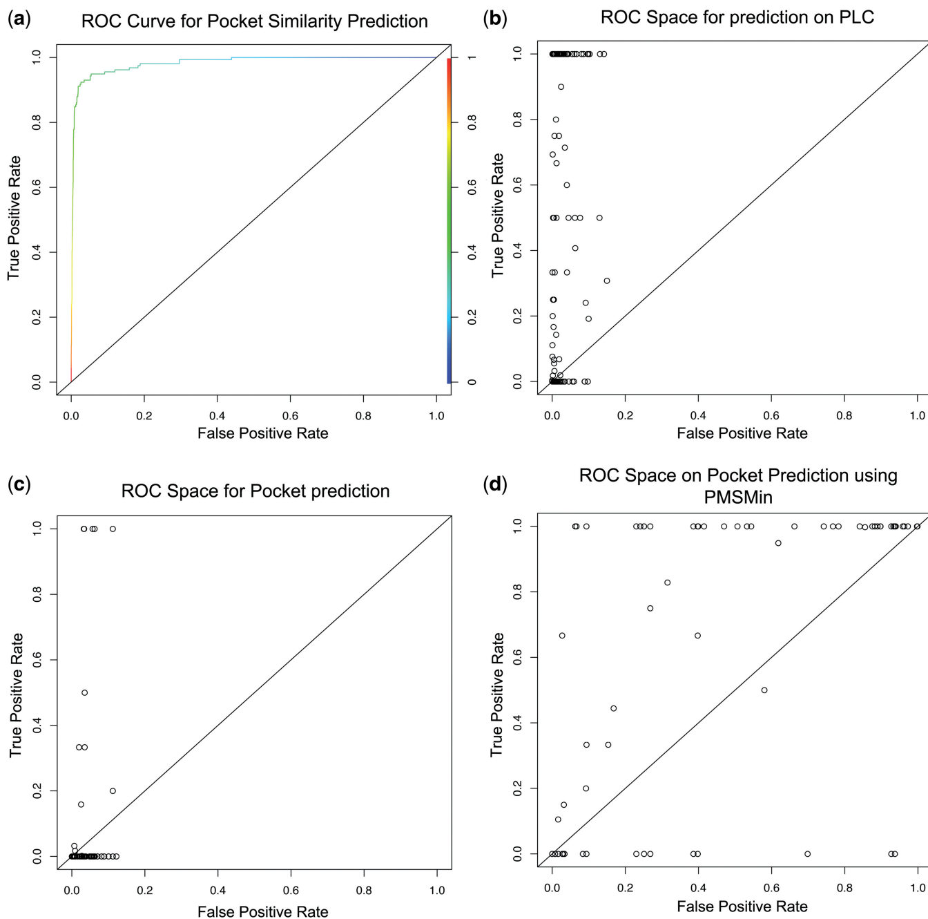
Figure 5. Sensitivity and specificity analyses. (a) ROC curve obtained for pocket similarity prediction of sites extracted from 98 protein–ligand complexes (holo form). (b) ROC space of each of prediction made for the hit against the database by considering each binding site of protein–ligand complex (holo form). (c) ROC space for the pockets predicted by the PocketDepth on corresponding set of apo proteins. (d) ROC space for the pockets by considering PMS_{MIN} scores for the PocketDepth predictions on apo-form of proteins.
