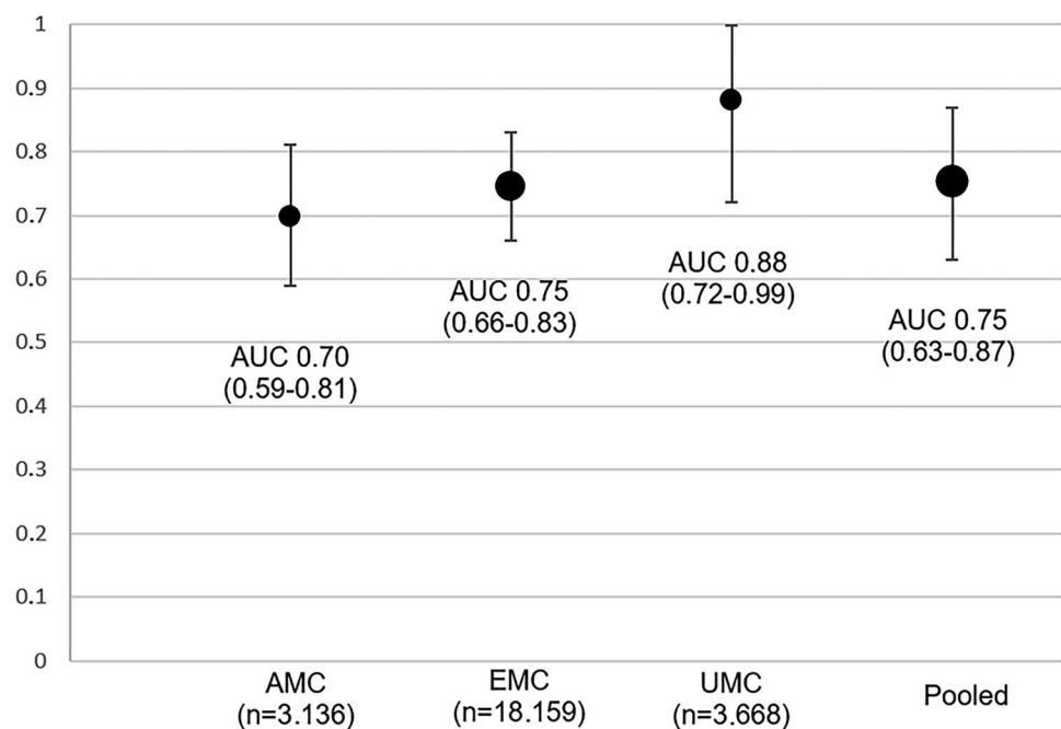
Fig. 1 Discriminative value (AUC with 95% confidence intervals) of the reduced model for the consensus diagnosis of child maltreatment for 3 internal–external cross-validations. Unknown outcomes of the screened negatives are analysed as negative outcome (outcome measure A)
