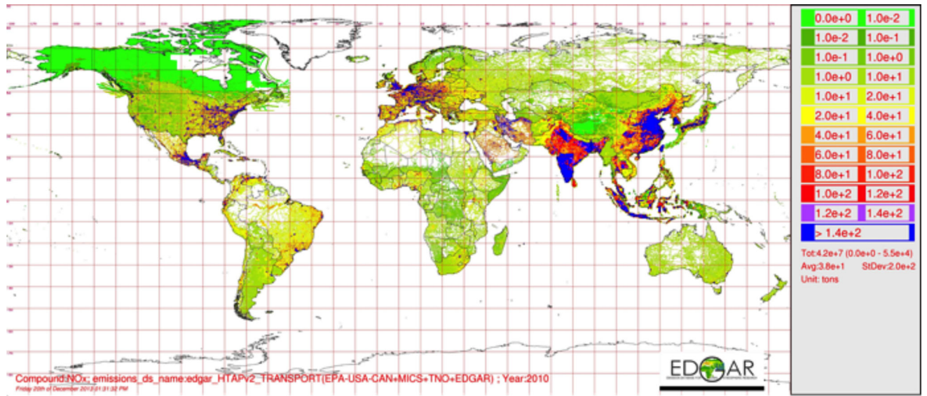
Figure 1. Example of HTAP_v2.2 emission mosaics for NO x in the transport sector.
