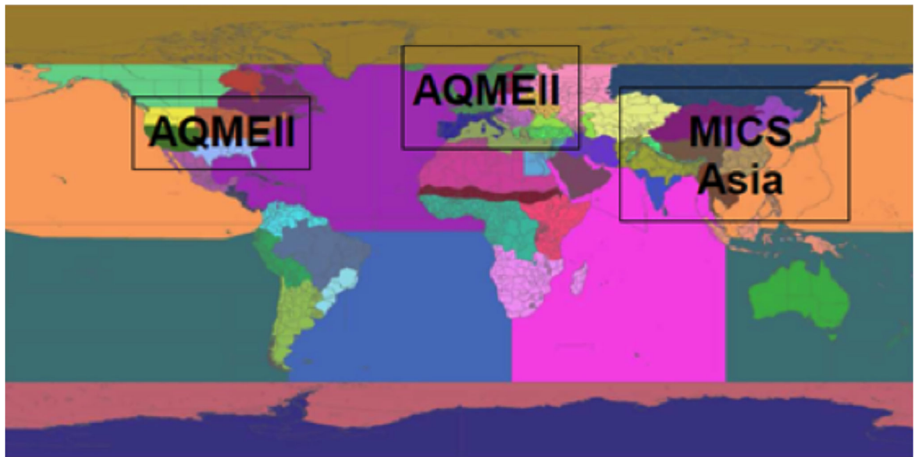
Figure 3. Domains of the regional model simulations and source/receptor areas.
