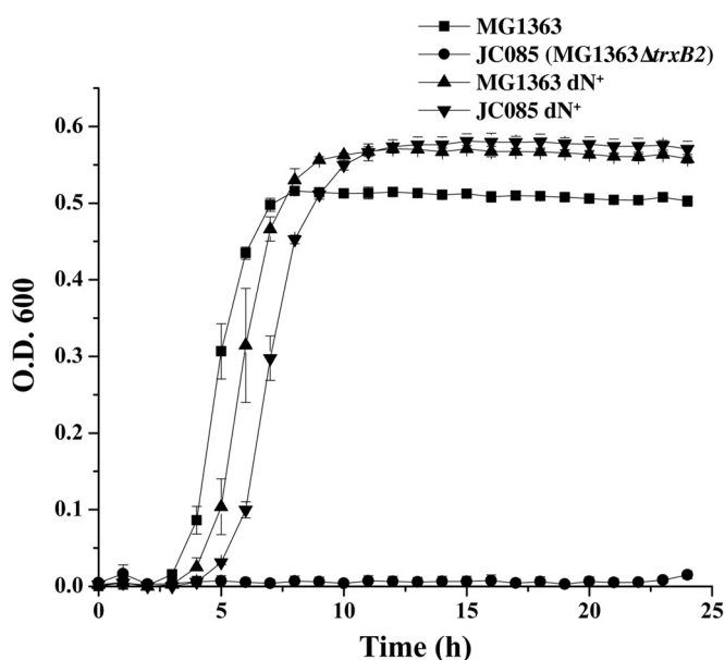
FIG 6 Positive effect on growth of the \Delta trxB2 mutant of deoxynucleosides. The wild-type MG1363 and its trxB2 deletion derivative (JC085) were characterized in liquid M17 medium using a Bioscreen. Cultures to which deoxynucleosides were added are indicated with “dN+.” For further information regarding growth conditions, see Materials and Methods.
