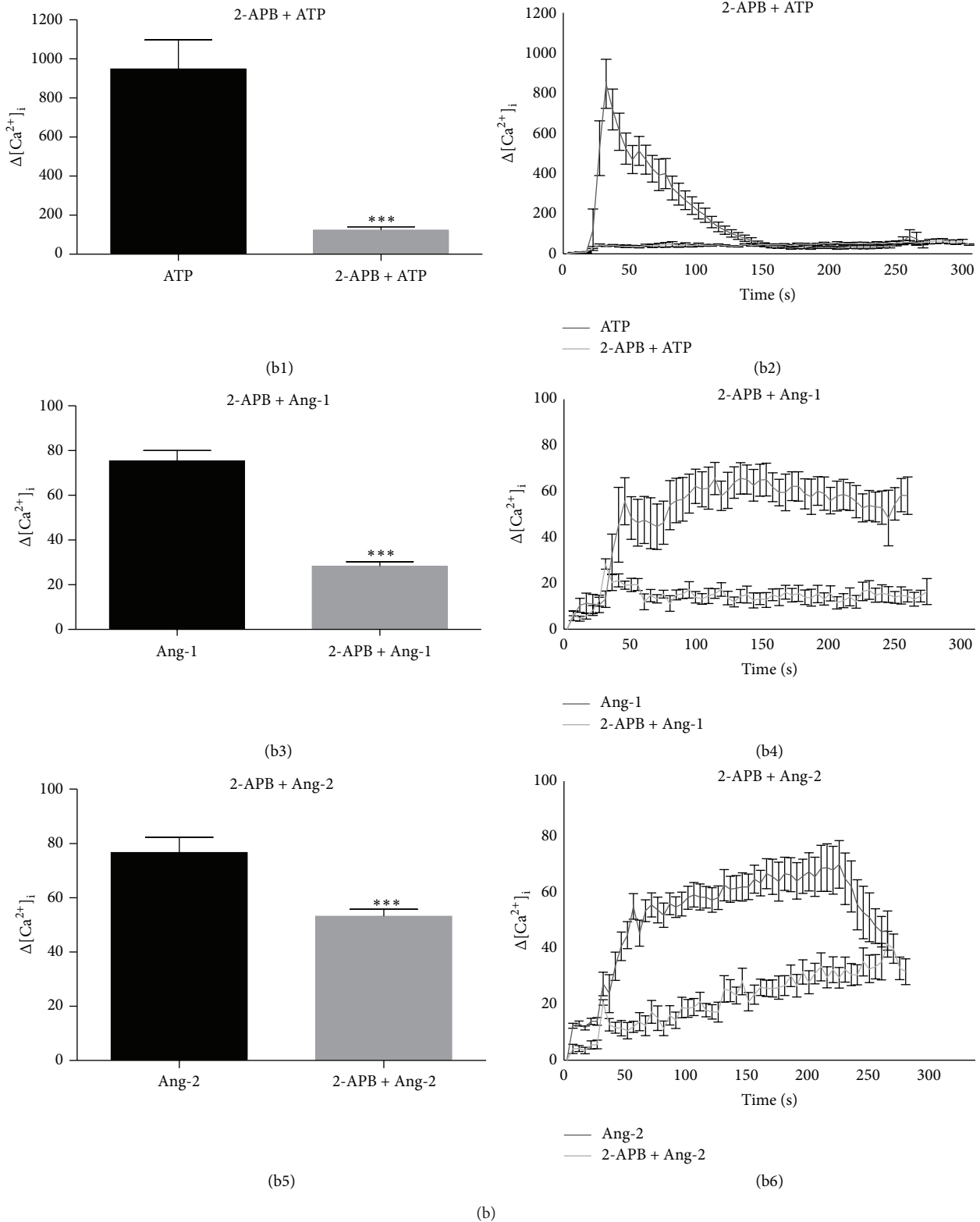
FIGURE 3: Ang-1- and Ang-2-dependent [Ca^{2+}]_i mobilization is inhibited by antagonists of PLC and of IP_3R . Cells pretreated for 20 min with 2\ \mu M U73122 (antagonist of PLC) or U73343 (its nonfunctional analogue) and cells pretreated for 30 min with 75\ \mu M 2-APB (selective antagonist of IP_3 receptor) were stimulated with 10\ \mu M ATP (positive control) or Angs in Ca^{2+} -free medium KHH. Statistical evaluation of \Delta[Ca^{2+}]_i in response to each agonist in the presence or absence of the indicated inhibitors (a1, a3, a5, b1, b3, and b5). Changes in [Ca^{2+}]_i levels are shown as representative traces indicating the effect of U73122/U73343 or 2-APB on cells stimulated with ATP or Ang-1 or Ang-2 in Ca^{2+} -free medium (a2, a4, a6, b2, b4, and b6). \Delta on the y-axes = nM. Data in bar charts represent mean \pm s.e.m. from three independent experiments. Cell number = 88–140. *** P < 0.001 versus agonists by Student's t -test. [Ca^{2+}]_i values in representative traces are expressed as increase with respect to basal Ca^{2+} concentrations ( \Delta ).
