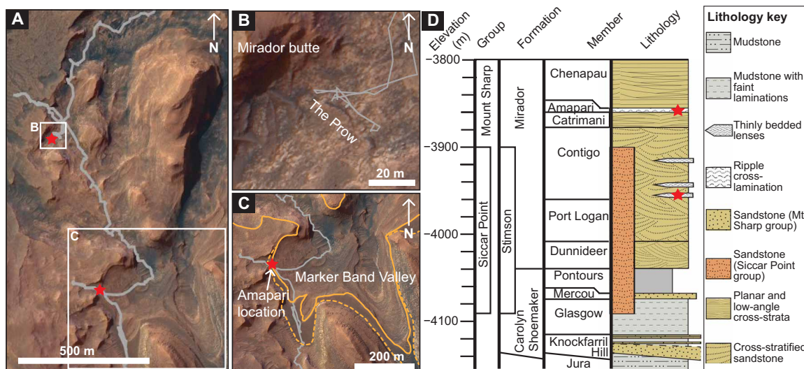
Fig. 1. Location of the Amapari Marker Band and Prow outcrops. Along the Curiosity traverse [(A), gray line] through the Mirador formation, the rover observed symmetric ripple marks within the Prow outcrop near the base of Mirador butte at elevation -3950 m (B) and the Amapari Marker Band (AMB) outcrop along the west side of Marker Band Valley (MBV) at elevation -3860 m (C). Red stars indicate the locations of the ripple-containing outcrops within the stratigraphic column (D) along the MSL traverse (A). The Prow is one of the multiple lenticular outcrops within the Contigo member. The AMB outcrops are nearly continuously around MBV [(C): solid orange line], often forming flat, erosionally resistant benches (inner edge traced in dashed orange line). The basemap used in (A) to (C) is a Mars Reconnaissance Orbiter HiRISE mosaic generated by Calef et al. (61, 62) and accessed through the NASA Planetary Data System.
