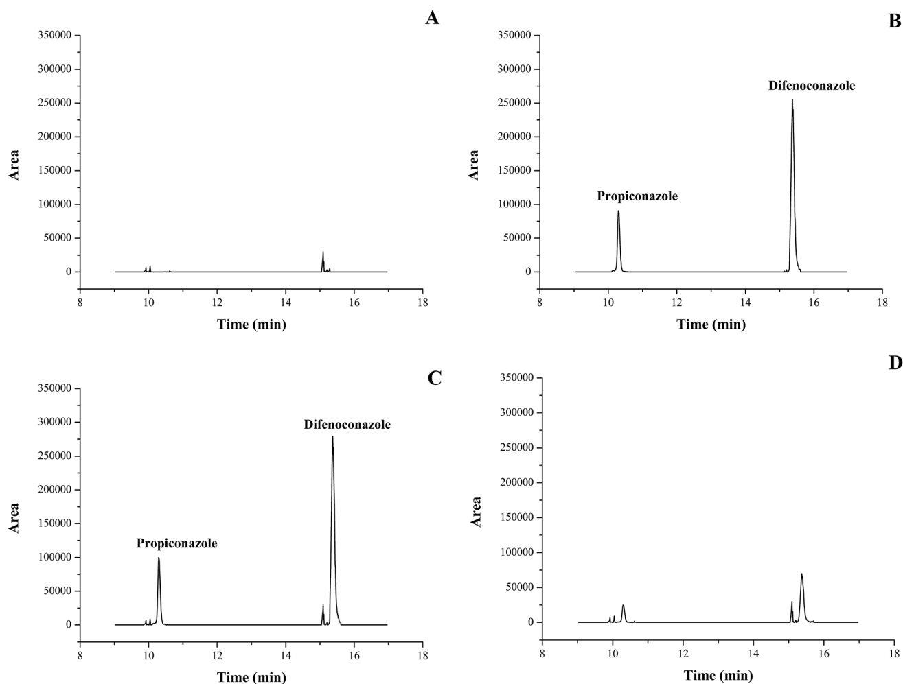
Fig. 3 Typical GC-MS/MS chromatograms of difenoconazole and propiconazole: (A) blank leaf sample, (B) standard solution (0.02 \mu\text{g mL}^{-1} ), (C) matrix-matched standard solution (0.02 \mu\text{g mL}^{-1} ) and (D) leaf spiked sample (0.02 mg kg -1 ).
