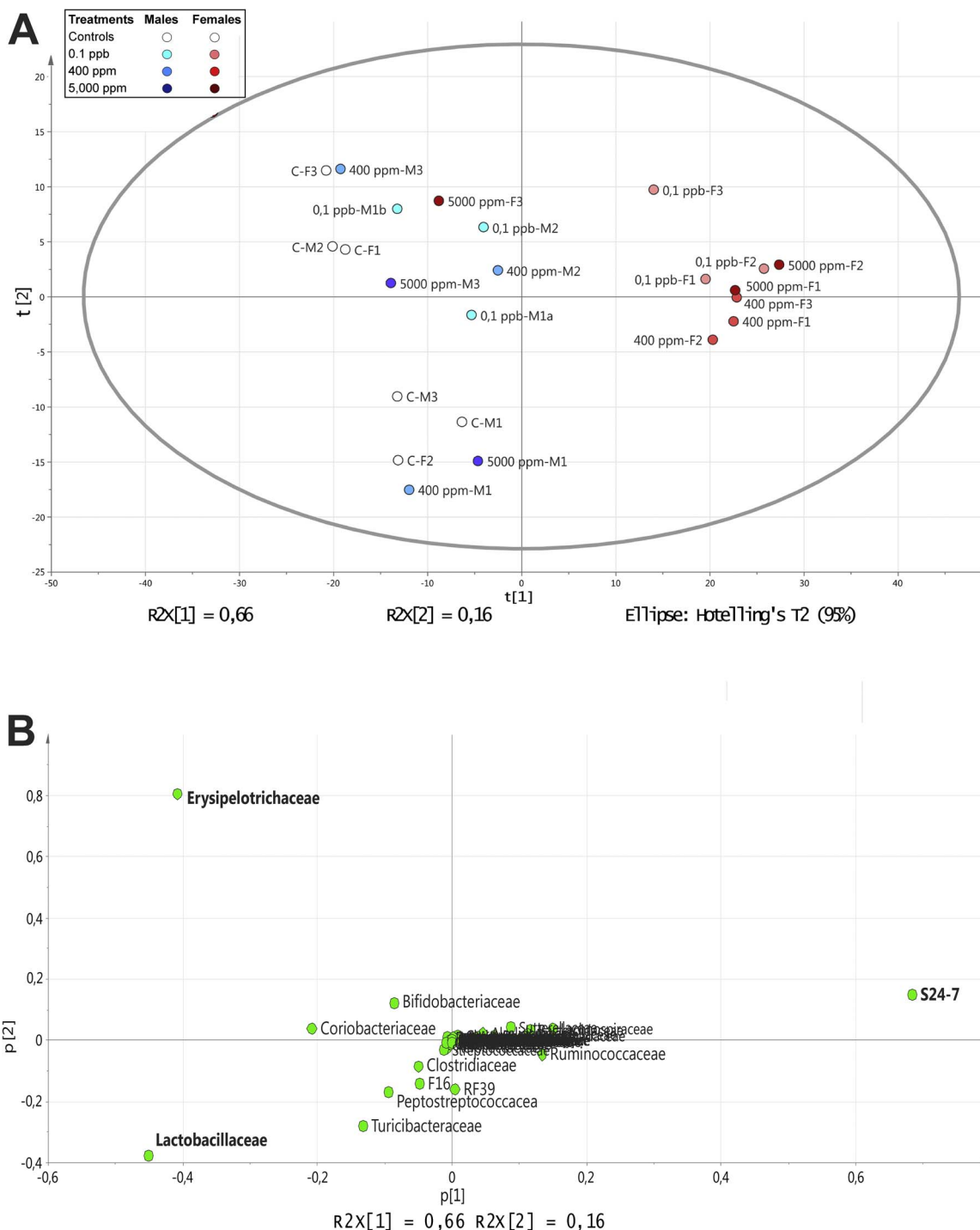
Fig. 2. Family-level gut microbiome profile of Roundup-treated rats. Feces from males and females rats chronically administered with R at three different concentrations (0.1 ppb R, 50 ng/L G; 400 ppm R, 0.1 g/L G; 5000 ppm R, 2.25 g/L G) were studied by high-throughput IonTorrent 16S sequencing analysis. (A) PCA score plot of the refitted model of families. (B) Loading plot of the refitted PCA model of families.
