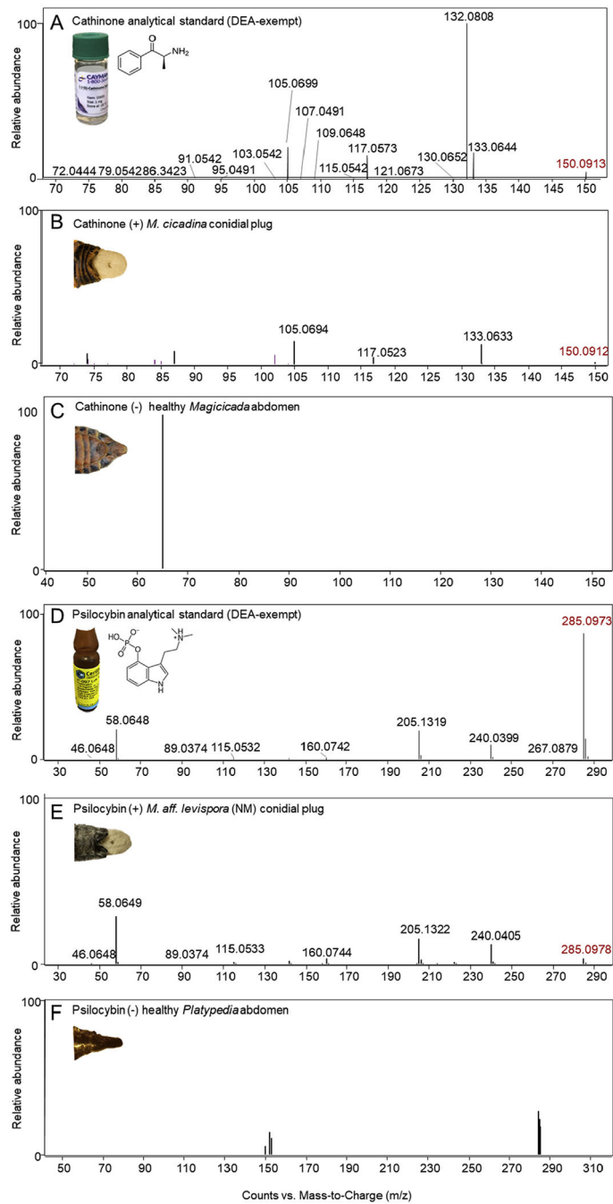
Fig. 4. Representative LC-MS/MS spectra for (A) cathinone DEA-exempt analytical standard; (B) cathinone-positive Mas. cicadina conidial plugs from infected Magicicada spp.; (C) cathinone-negative Magicicada septendecim abdominal sample; (D) psilocybin DEA-exempt analytical standard; (E) psilocybin-positive Mas. aff. levispora (NM) conidial plugs from infected Platypedia putnami ; (F) psilocybin-negative Platypedia putnami abdominal sample. M/z in red denote precursor fragment while m/z in black denote observed fragments. All
