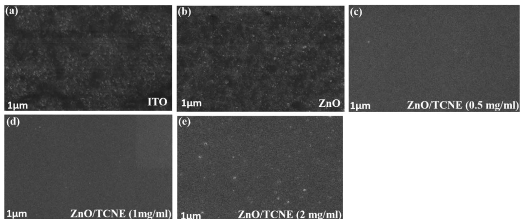
Fig. 7 Top view SEM images of (a) bare ITO, (b) ZnO, (c–e) different TCNE concentrations (as 0.5 \text{ mg ml}^{-1} , 1 \text{ mg ml}^{-1} , and 2 \text{ mg ml}^{-1} ) coated on ZnO film.
