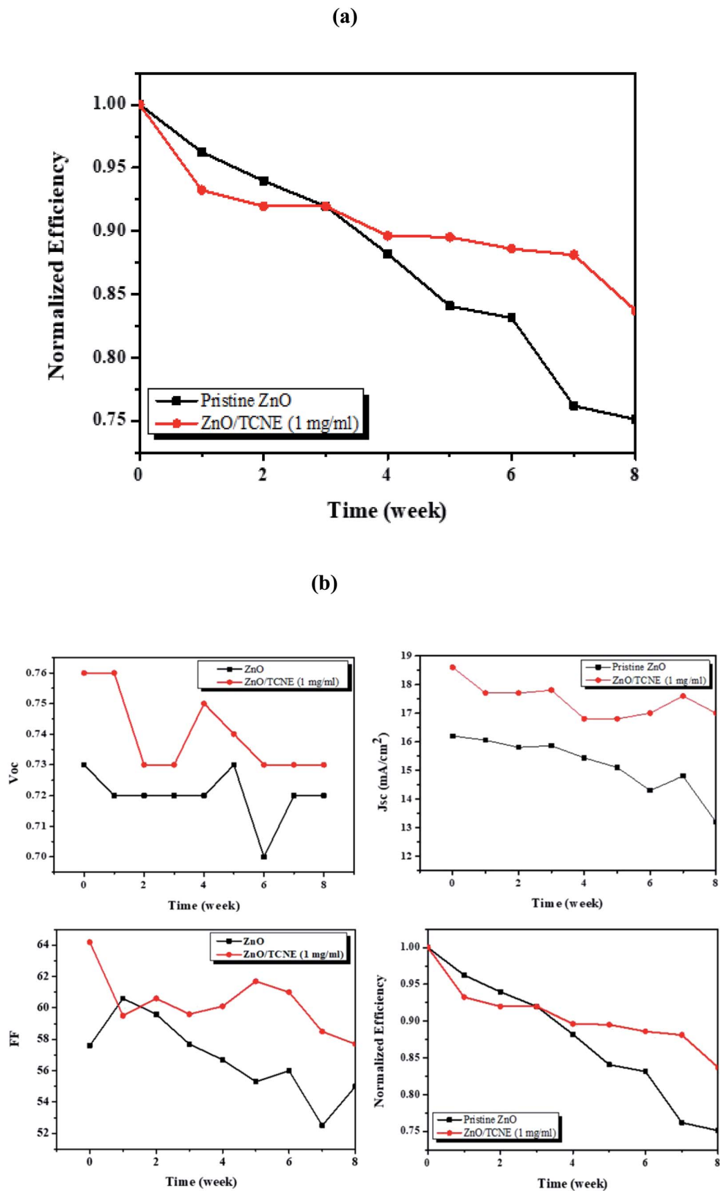
Fig. 10 (a) Normalized power conversion efficiencies of ZnO and ZnO/TCNE ETLs, respectively, devices as a function of eight weeks of storage time (b) I - V parameter breakdown of V_{oc} , J_{sc} , FF, and PCE vs. time in eight weeks.
