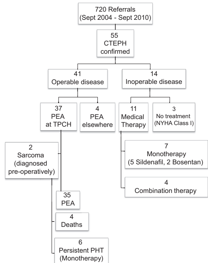
Figure 2: Study flowchart.
