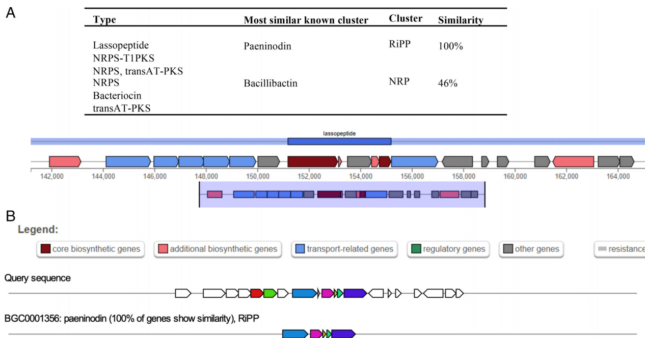
Fig. 6. Secondary metabolite prediction in strain S150 assessed with antiSMASH. A. Type of cluster and most similar one. B. Homologous gene cluster.
