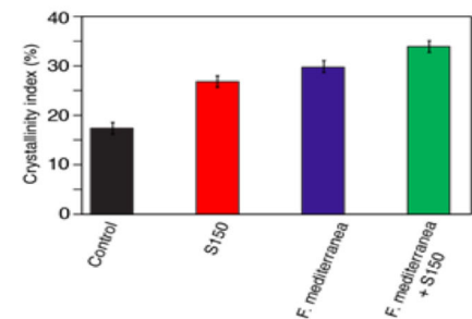
Fig. 3. Wood decay characterization after 8 months of incubation in Petri plates with Fmed (Fm) and Paenibacillus sp. (S150), alone or in combination, compared to a control without microorganisms.
