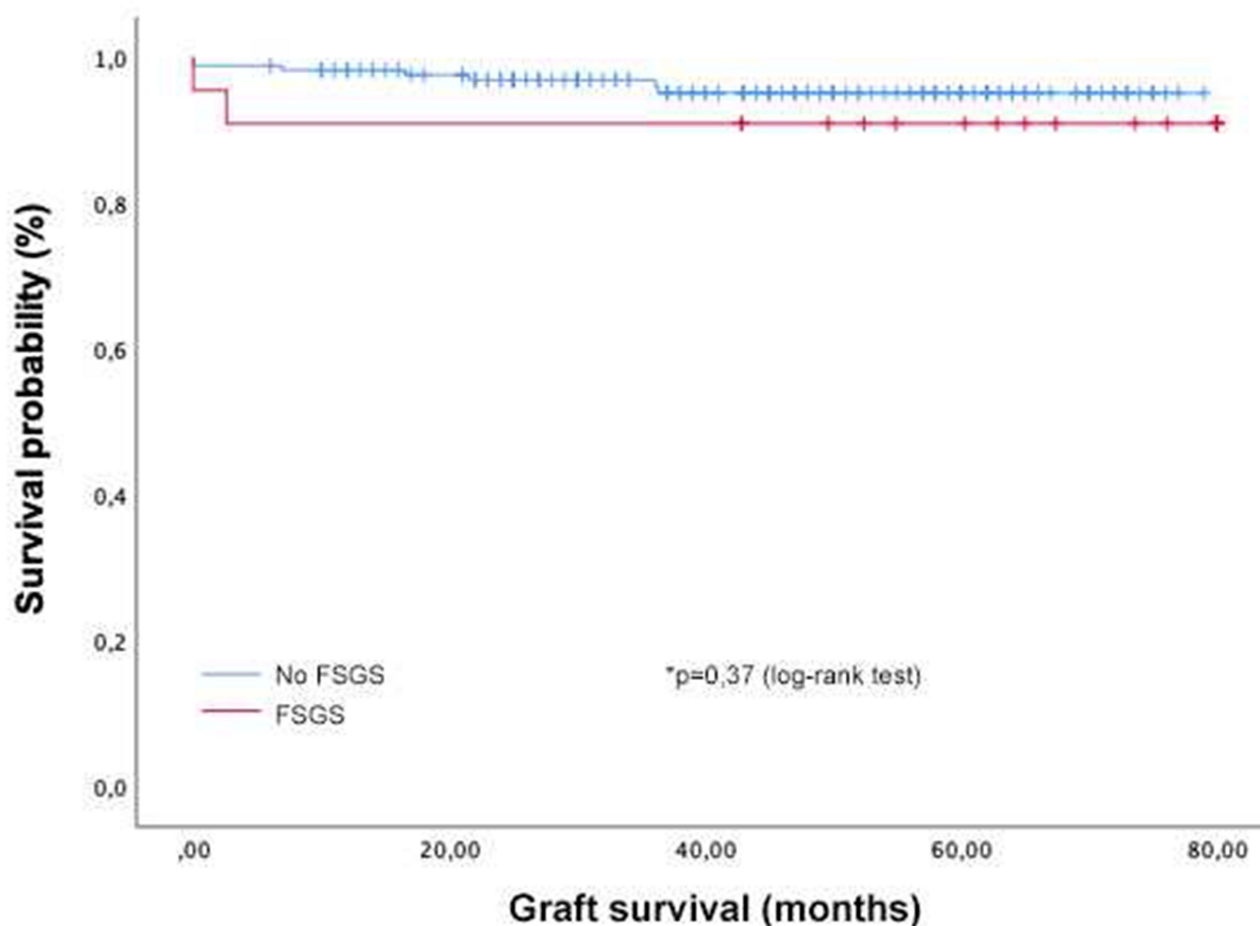
Figure 1 Kaplan-Meier Analysis.
