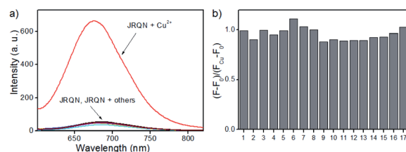
Fig. 2 (a) Fluorescence emission responses of JRQN (10 \mu\text{M} ) upon addition of different species; (b) fluorescence ratio ((F - F_0)/(F_{\text{Cu}} - F_0)) changes of JRQN in the presence of 100 \mu\text{M} \text{Cu}^{2+} and different species. Metal cations (100 \mu\text{M} ): (1) \text{Ag}^+ ; (2) \text{Al}^{3+} ; (3) \text{Ca}^{2+} (10 mM); (4) \text{Cd}^{2+} ; (5) \text{Co}^{2+} ; (6) \text{Cr}^{3+} ; (7) \text{Cu}^{2+} ; (8) \text{Fe}^{2+} ; (9) \text{Fe}^{3+} ; (10) \text{Pd}^{2+} ; (11) \text{K}^+ (10 mM); (12) \text{Li}^+ (10 mM); (13) \text{Mg}^{2+} (10 mM); (14) \text{Mn}^{2+} ; (15) \text{Na}^+ ; (16) \text{Ni}^{2+} ; (17) \text{Zn}^{2+} . The conditions: HEPES buffer (10 mM, pH = 7.4, containing 20% \text{CH}_3\text{CN} ), \lambda_{\text{ex}} = 580 \text{ nm} , slit = 5/5 nm.
