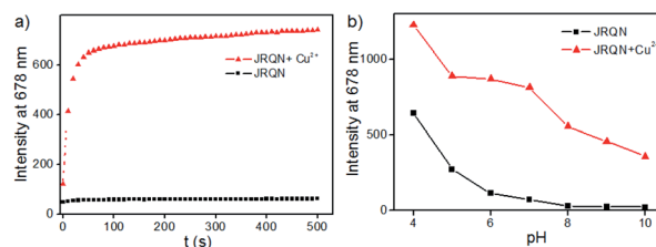
Fig. 4 (a) Time-dependence fluorescence intensity of JRQN (10 \mu\text{M} ) upon addition of 100 \mu\text{M} \text{Cu}^{2+} ; (b) fluorescence intensity of JRQN (10 \mu\text{M} ) as a function of pH value in the absence/presence of \text{Cu}^{2+} (100 \mu\text{M} ); the conditions: HEPES buffer (10 mM, pH = 7.4, containing 20% \text{CH}_3\text{CN} ), \lambda_{\text{ex}} = 580 nm, slit = 5/5 nm.
