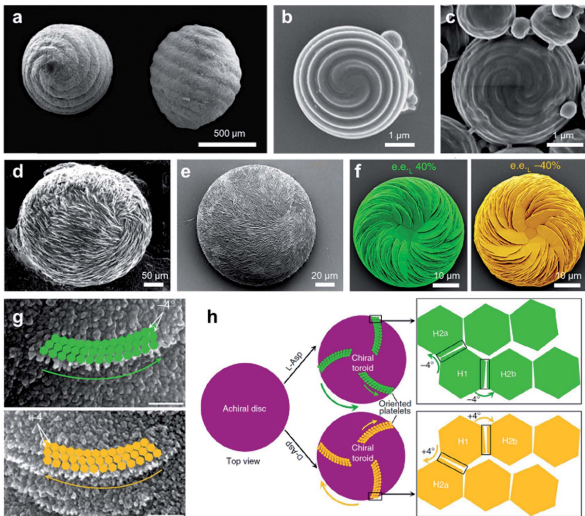
Fig. 11 Biomimetic synthesis of hierarchical chiral structures via self-assembly. (a) Charophyte gyrogonites from the Huchpayacu formation, Contamana, and Peruvian Amazonia in (left) basal and (right) lateral views. Reproduced from ref. 144 with permission from Elsevier Ltd, copyright 2016. (b and c) SEM images of particles with opposite chiral spiral morphologies. (b and c) Reproduced from ref. 145 with permission from American Chemical Society, copyright 2018. (d) Rounded, chiral pathologic calcium carbonate vaterite otoconia from the inner ear of an aged. Reproduced from ref. 147 with permission from Elsevier Ltd, copyright 1982. (e) Synthetic chiral suprastructure of hierarchically organized vaterite induced by the amino acid L-Asp as prepared in the lab. Reproduced from ref. 146 with permission from American Association for the Advancement of Science, copyright 2018. (f) SEM images of vaterite helicoids showing chiral vaterite platelets having counterclockwise or clockwise orientation when L- or D-Asp is the majority enantiomer under nonracemic solution conditions, respectively. Reproduced from ref. 149 with permission from Nature Publishing Group, copyright 2019. (g) High-magnification SEM images of chiral toroid platelets showing tilting of nanoparticle (nanohexagon) growth induced by selective chiral amino-acid adsorption. This chirality-inducing effect causes rounded/curved platelet edge growth having either a counterclockwise direction for L-Asp (green arrows) or a clockwise direction for D-Asp (yellow arrows). (h) Tilting mechanism leading to the formation of chiral vaterite toroids. (g and h) Reproduced from ref. 148 with permission from Nature Publishing Group, copyright 2017.
