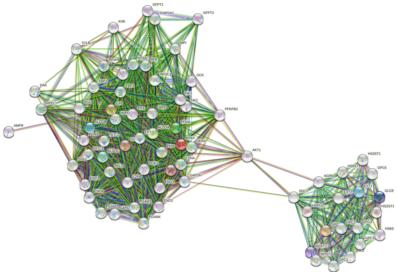
Figure 4 The interacting genes of PFKP and GPC6 were displayed by String software.
