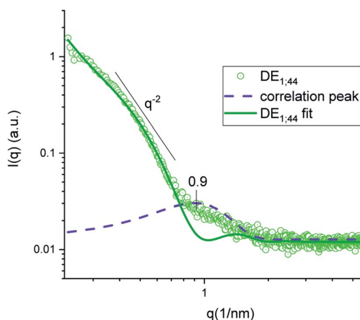
Fig. 4 SAXS intensity of sample DE_1 stored at room temperature fitted by a polydisperse bilayer model (green), with Gaussian peak (violet) superposition to account for inter-bilayer correlation.
