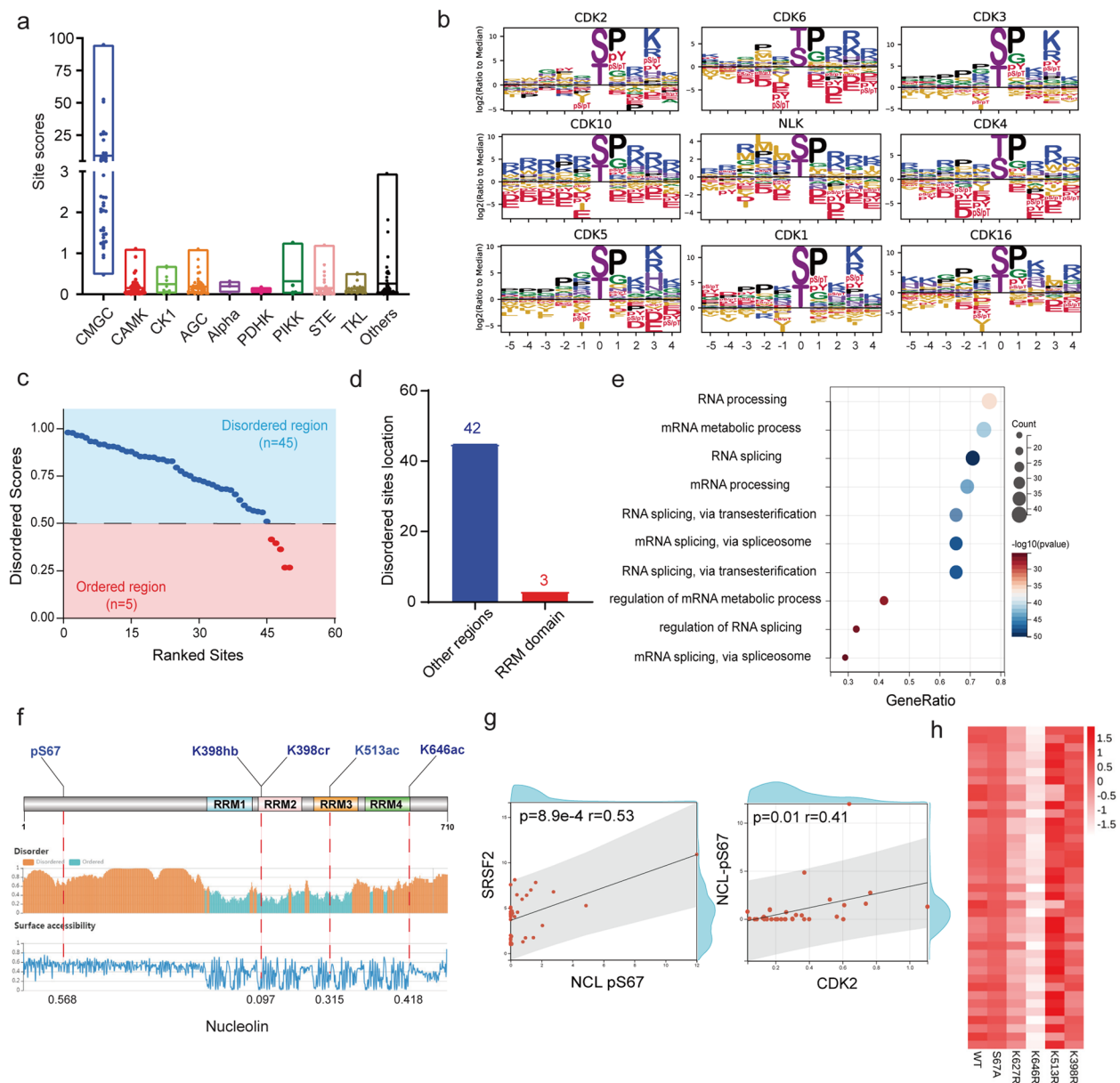
Fig. 5 Regulatory patterns in the phosphorylation of RRM1-containing proteins. a Kinase scoring showing potential kinases at the phosphorylation sites on RRM1-containing proteins. The scores are calculated via the GPS algorithm to evaluate the potential for phosphorylation. The higher the value is, the more potential the residue is phosphorylated. b Icelogos showing the percent difference in amino acid frequency at each position for the top 9 kinase-regulated sites compared with unregulated sites, with a P value cutoff of 0.05. Filled logos show the fraction of each amino acid in positions flanking the regulated sites. c Ranked abundance points represent disordered z scores of phosphorylated sites; phosphorylated sites with z scores > 0.5 are defined as sites located in disordered regions, and phosphorylated sites with z scores < 0.5 are defined as sites located in folded regions. d Bar chart showing the counts of phosphorylated sites in RRM1-containing proteins located in IDRs and folded regions. e Enriched bubble plot showing biological process enrichment in phosphorylated RRM1-containing proteins. f The secondary structure of nucleolin shows a modified site distribution on nucleolin. g Spearman's correlation coefficient showing a positive relationship between the modified abundance of NCL-pS67 and the expression level of SRSF2 or CDK2. h Heatmap showing the interaction propensity of NCL-WT, NCL-S67A, NCL-K627R, NCL-K398R, NCL-K646R, and NCL-K513R. The scores of interaction propensity are calculated via catRAPID 2.0
