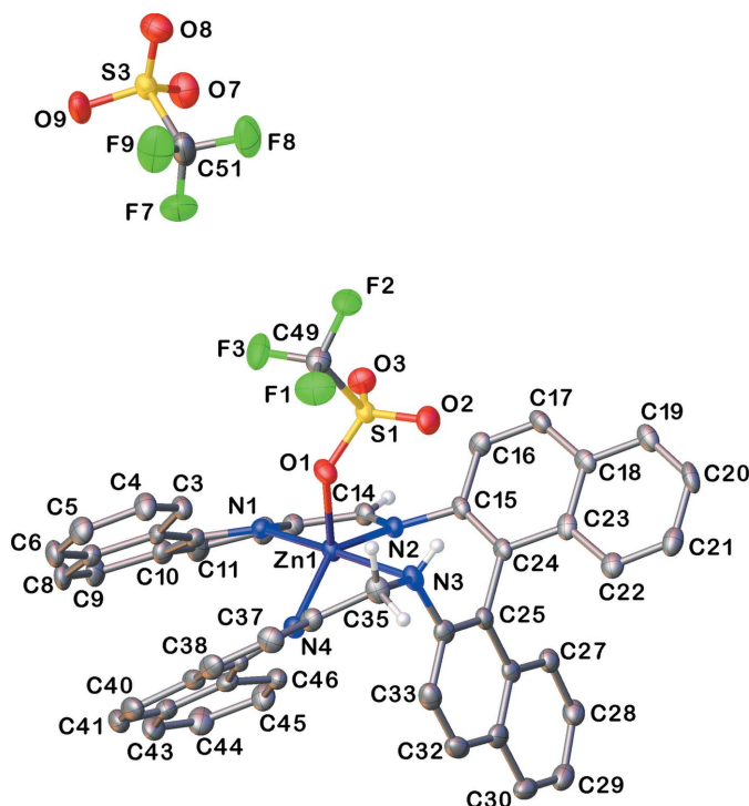
Figure 1 The molecular structure for one of the molecules of complex ( 1 ). Atomic displacement ellipsoids are depicted at the 50% probability level and H atoms are shown as spheres of arbitrary radius. All non-imine/amino H atoms and solvent molecules have been omitted for clarity.
