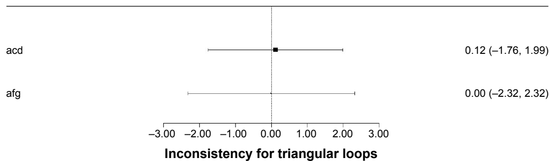
Figure 6 Inconsistency for triangular loops.
