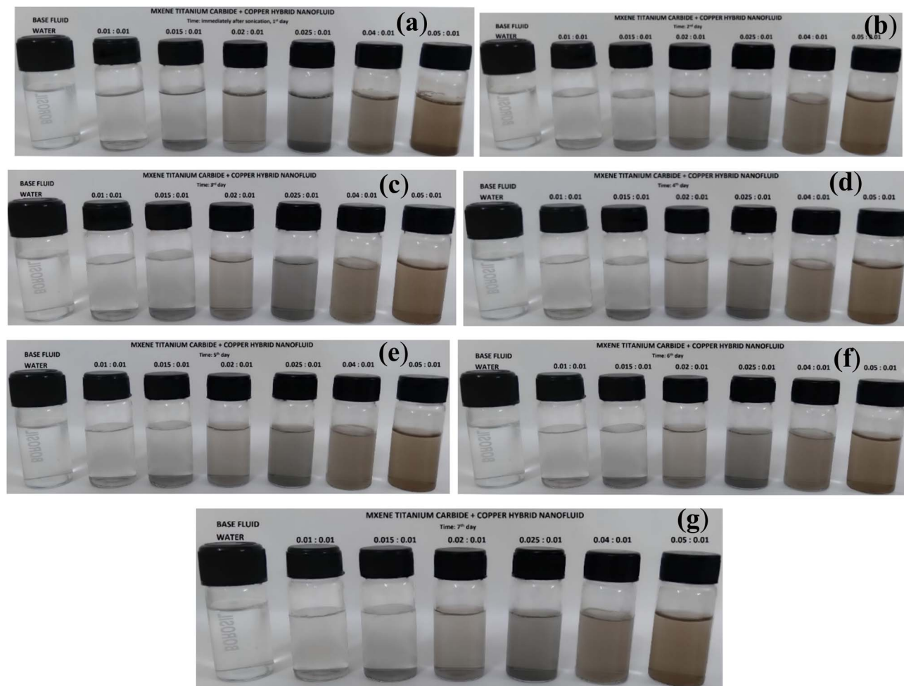
Fig. 9 Stability analysis of water based Cu-MXene hybrid nanofluids through visual inspection: (a) after preparation (b) after 2 days (c) after 3 days (d) after 4 days (e) after 5 days (f) after 6 days (g) after 7 days.
