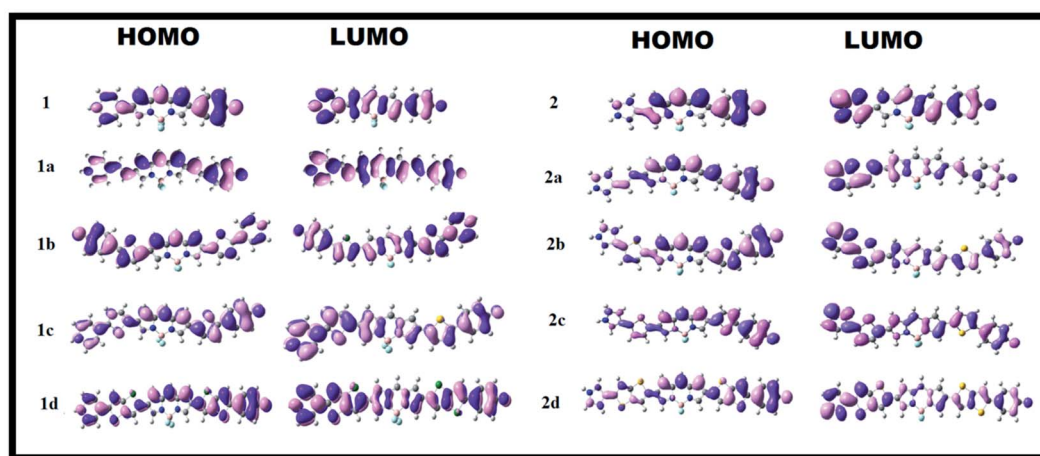
Fig. 3 Frontier molecular orbitals of the dyes in the gas phase at the B3LYP/6-311++G(d,p) level of theory.
