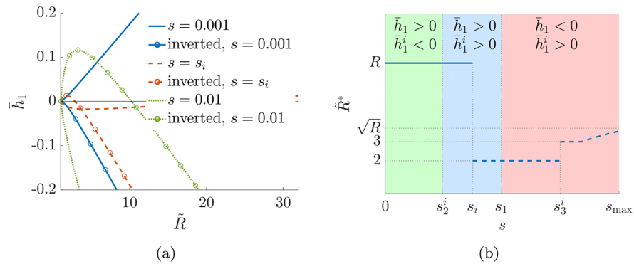
Fig 4. Panel (a) shows how depending on the value of s the inverted rank can give a higher value of \bar{h} than the planted rank in military-like graph with parameters p = 0.5, q = 0, R = 32 . Panel (b) gives a schematic representation of the estimated optimal number of classes \tilde{R}^* as s varies, dashed lines are associated to the inverted rank.
