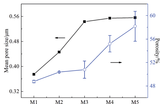
Fig. 8 Effects of on-line stretching ratio on the mean pore size and porosity.
