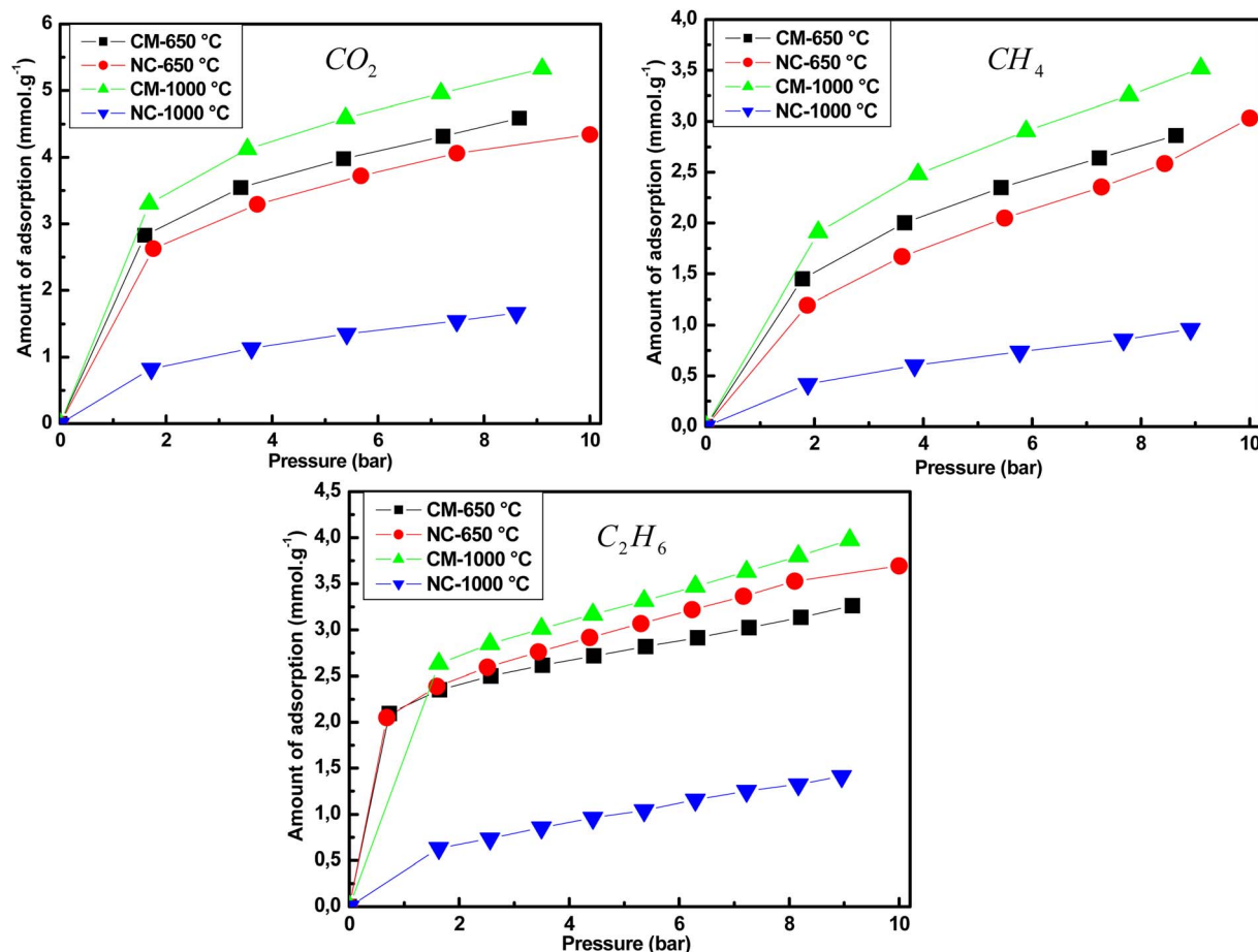
Fig. 12 Amount of adsorption of \text{CO}_2 , \text{CH}_4 and \text{C}_2\text{H}_6 for the different samples.
