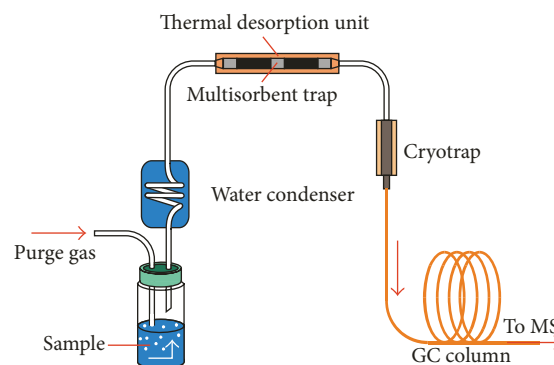
FIGURE 1: Diagram of analysis with online purge and trap-gas chromatography-mass spectrometry (PT-GC-MS).
