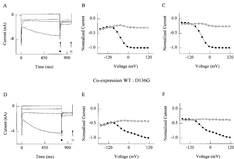
Each voltage step is followed by a fixed -105 -mV test pulse. (E) Voltage dependence of the instantaneous current amplitude (filled circles, I_{peak} ) and the current amplitude at the end of the -105 -mV test pulse (open squares, I_{ss} ) in WT:D136G co-transfected cells. (F) Current amplitudes corrected for the contribution of Cl^- currents conducted by D136G homomultimeric channels as described in the text.
