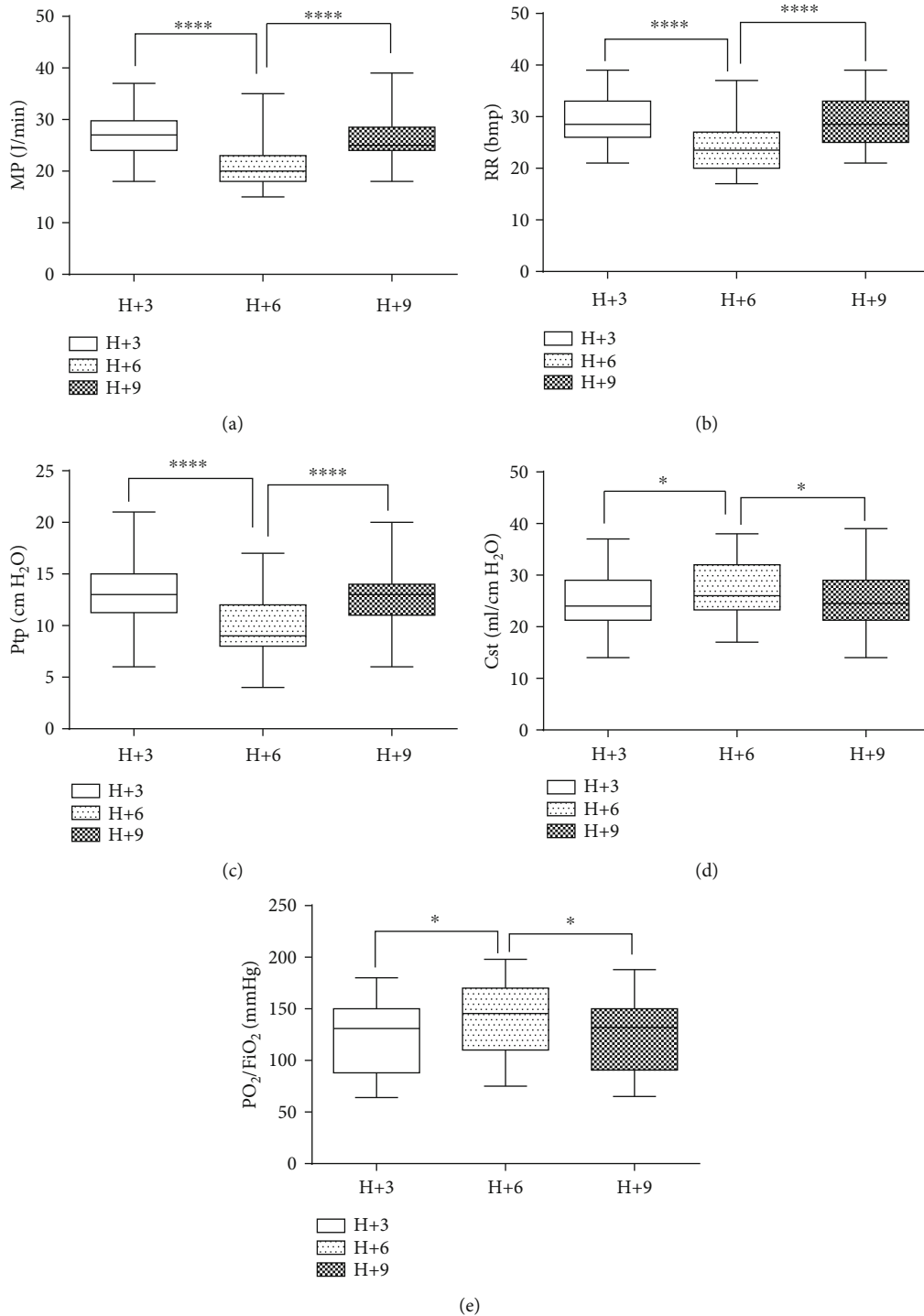
FIGURE 2: Parameter variation in ARDS patients under moderate to severe sedation. (a) MP. (b) RR. (c) Ptp. (d) Cst. (e) PF. Results were expressed as mean \pm standard deviation ( x \pm s ) of at least three different measurements. * P < 0.05 , **** P < 0.0001 .
