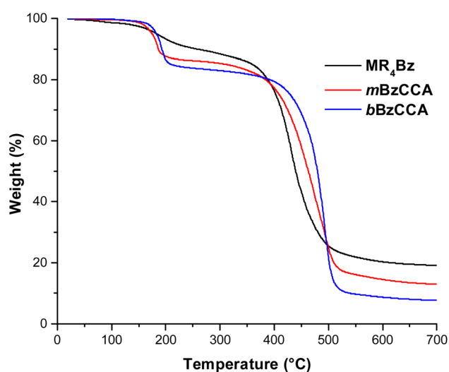
Fig. 4 Thermograms of \text{MR}_4\text{Bz} resin (black), m\text{BzCCA} (red) and b\text{BzCCA} (blue) obtained at 20\text{ }^\circ\text{C min}^{-1} under a \text{N}_2 atmosphere.
