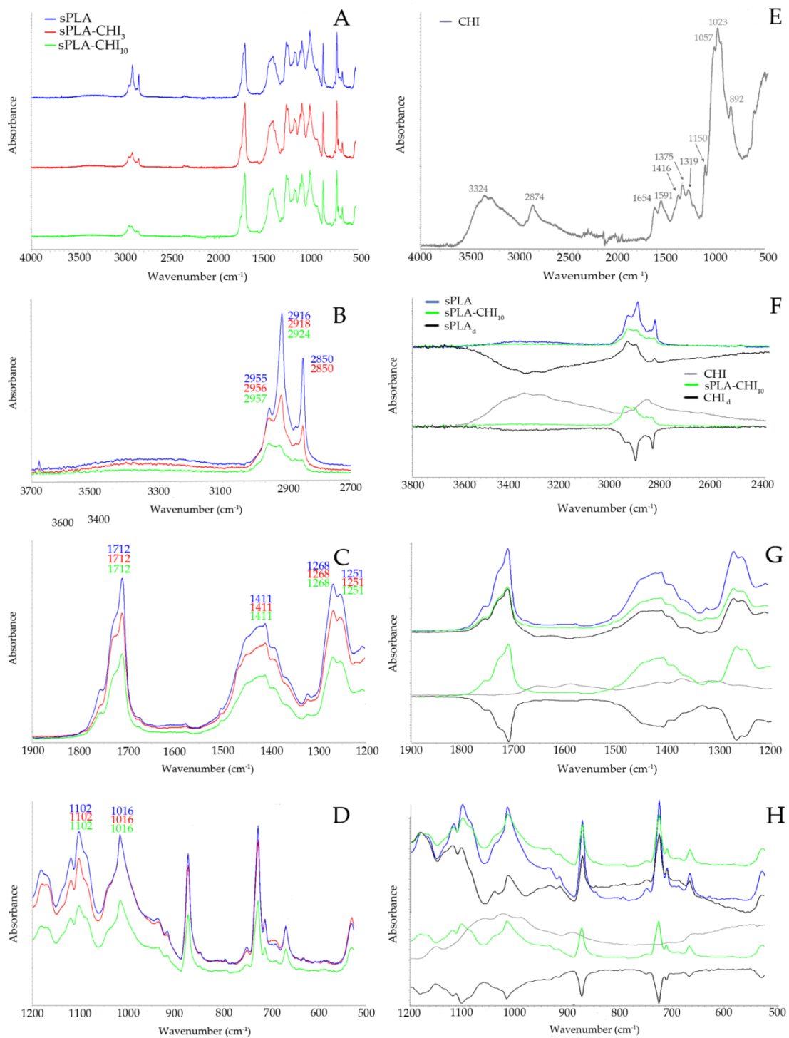
Figure 2. (A–D) FT-IR spectra of sPLA, sPLA-CHI 3 , sPLA-CHI 10 , (E) FT-IR spectrum of CHI; (F–H) FT-IR spectra of the sPLA, sPLA-CHI 10 , and difference spectrum of sPLA-CHI 10 from which the spectrum of CHI was subtracted (sPLA d ) on the top, FT-IR spectra of the CHI, sPLA-CHI 10 , and difference spectrum of sPLA-CHI 10 from which the spectrum of sPLA was subtracted (CHI d ) on the bottom. ((Different colored lines in B,C and D represent the same substance as A; different colored lines in G,H represent the same substance as F).
