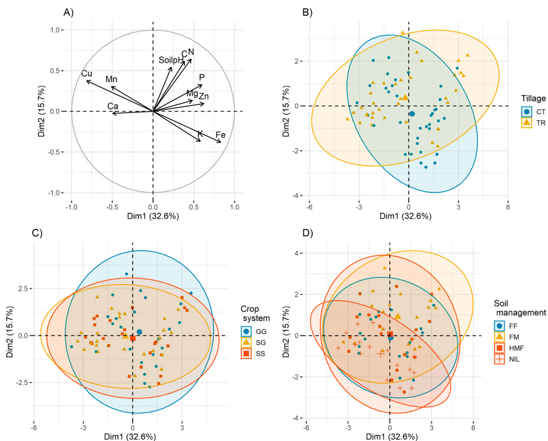
Fig. 6. Principle component biplots for soil parameters (Figure A) and individual plots with confidence ellipses for tillage, crop system and soil fertility management.
