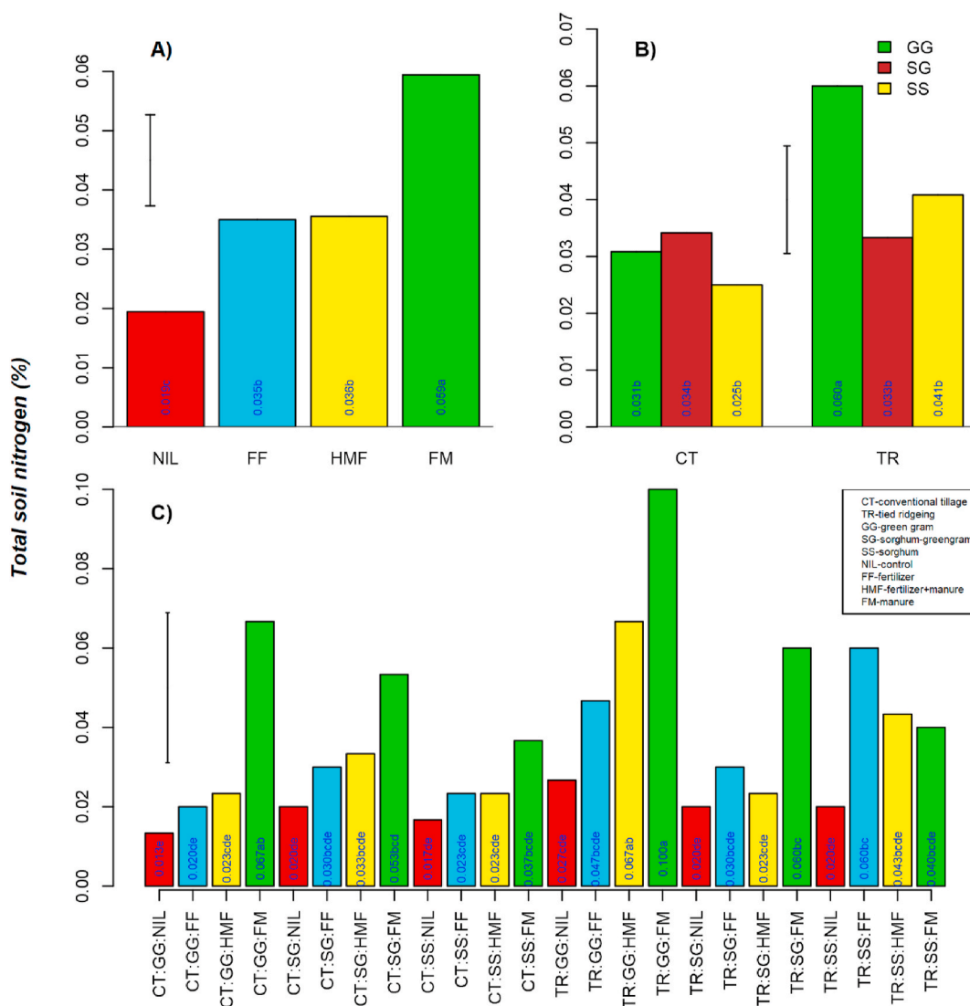
Fig. 2. Soil tillage, crop system, and fertility management effects on total soil N. Least significant differences are presented as error bars (A, -LSD fertility management, B-Tillage*Cropping interaction, C-Tillage*crop*fertility management interaction).
