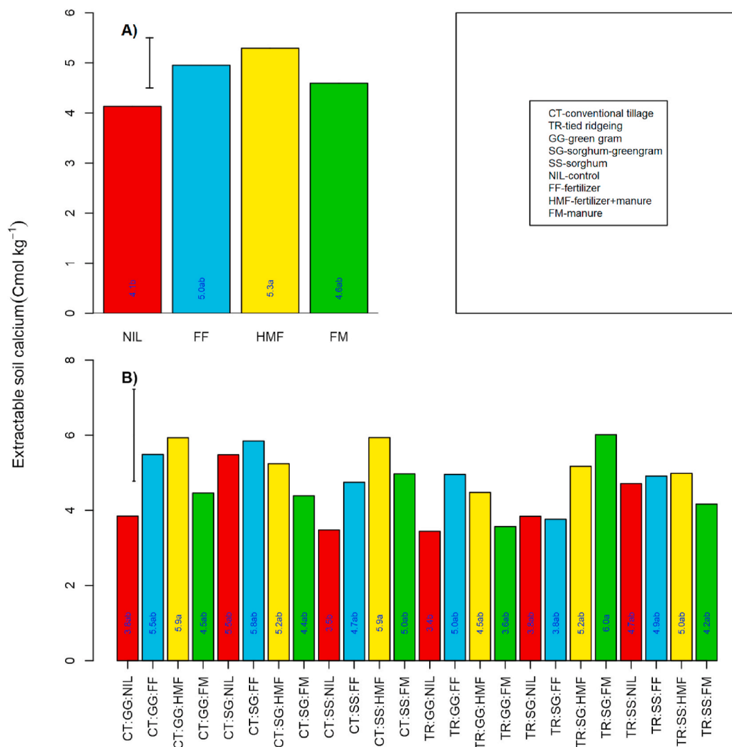
Fig. 4. Soil tillage, crop system, and fertility management effects on soil Ca. Means followed by the same letters are not significant. Least significant differences are presented as error bars (A,-LSD-soil fertility management, B-Tillage*crop*soil fertility management interaction).
