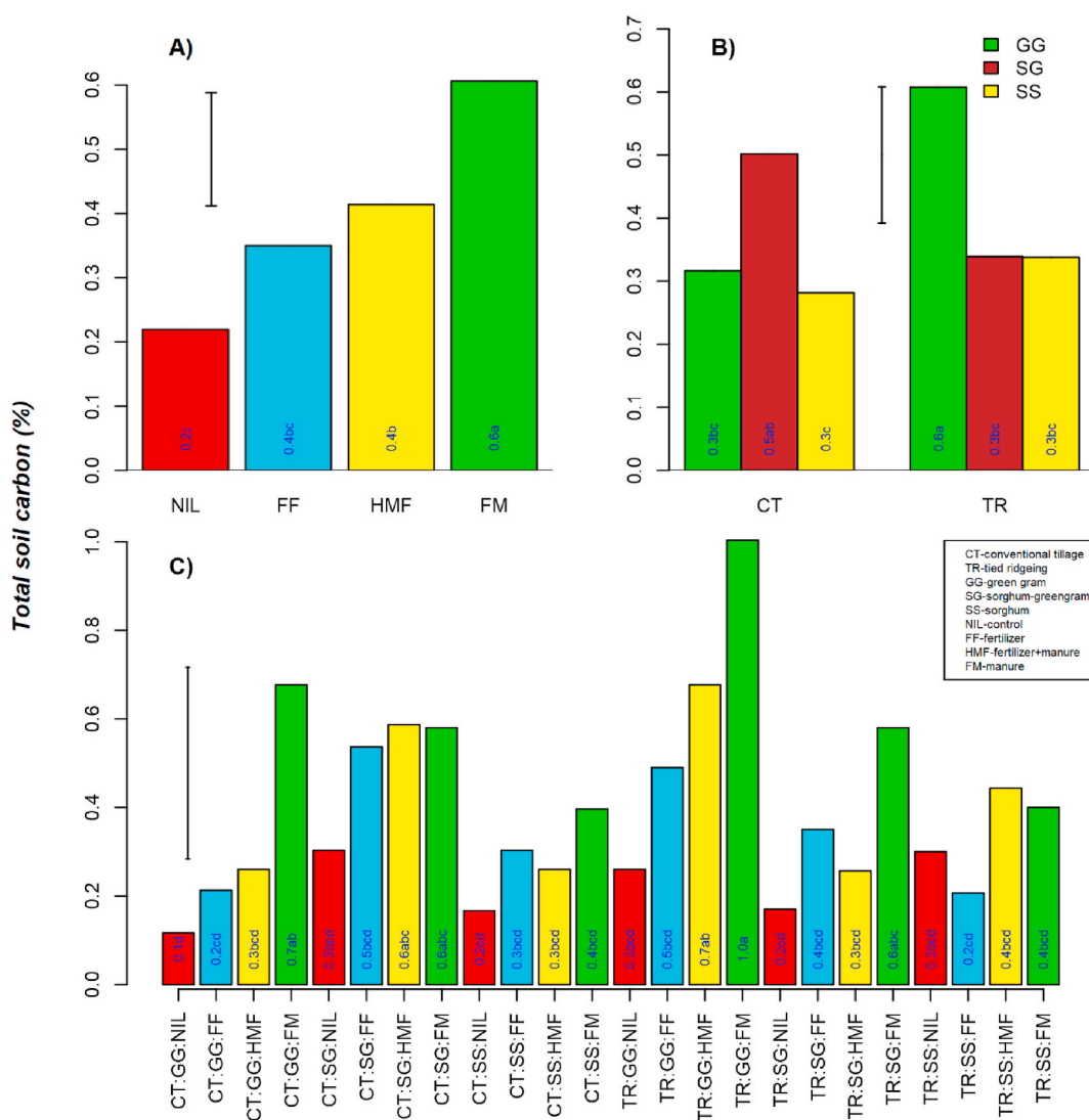
Fig. 1. Soil tillage, crop system, and fertility management effects on soil carbon. Means followed by the same letters are not significant. Least significant differences are presented as error bars (A,-LSD-soil fertility management, B-Tillage*Cropping, C-Tillage*crop*soil fertility management).
