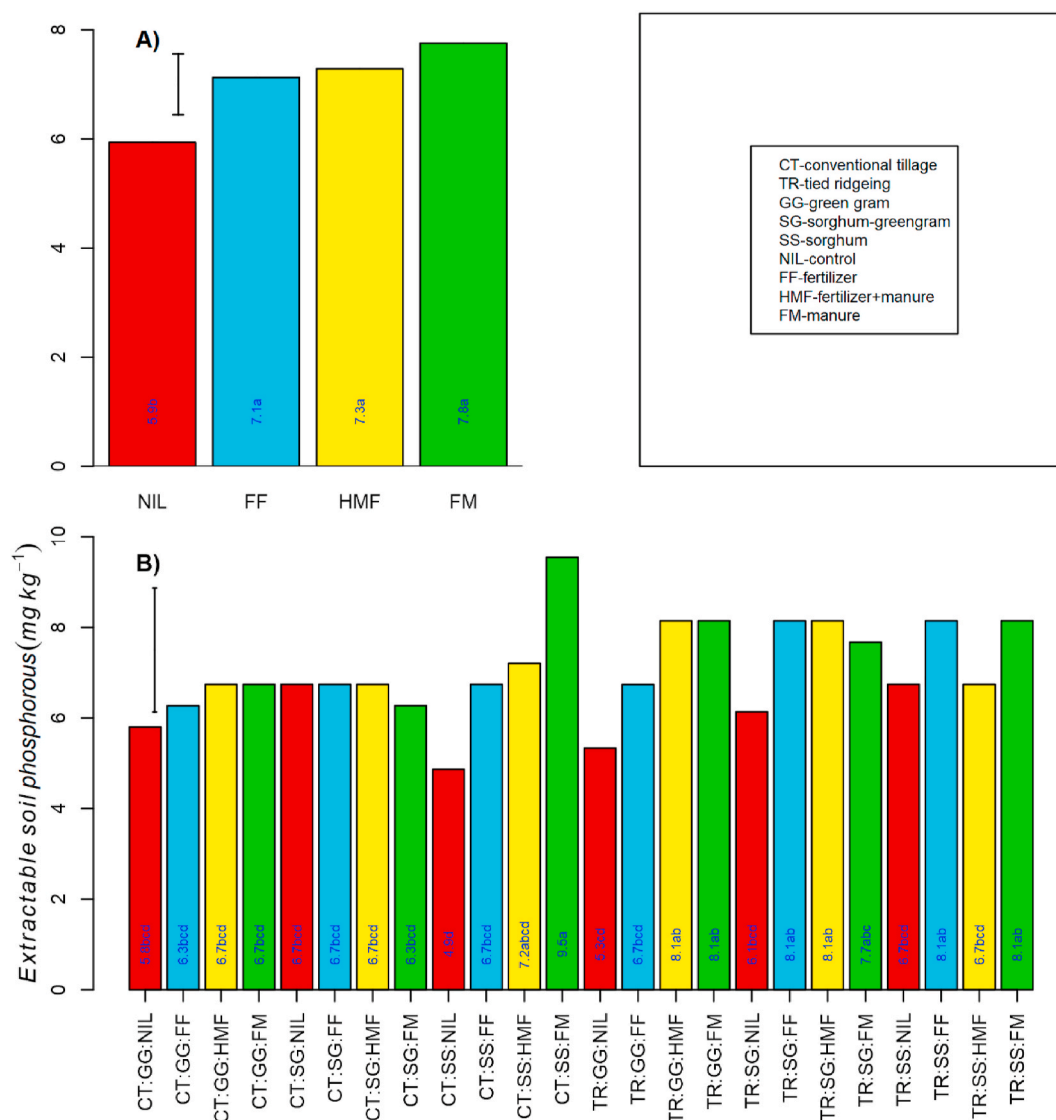
Fig. 3. Soil tillage, crop system, and fertility management effects on soil P. Means followed by the same letters are not significant. Least significant differences are presented as error bars (A, LSD-soil fertility management, B-Tillage*crop*soil fertility management interaction).
