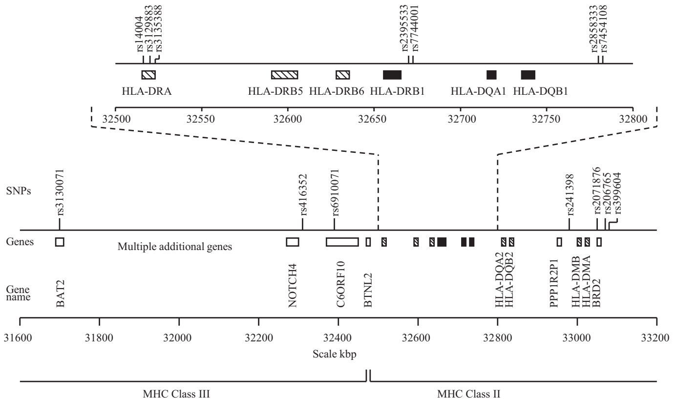
FIG. 1. Schematic diagram of the tag SNPs used for HLA haplotyping in the MHC region on chromosome 6 including nearby located genes. The HLA genes that are predicted by the tag SNPs are shown as black boxes; other HLA genes are shown as hatched boxes. Additional genes are shown as white boxes.
