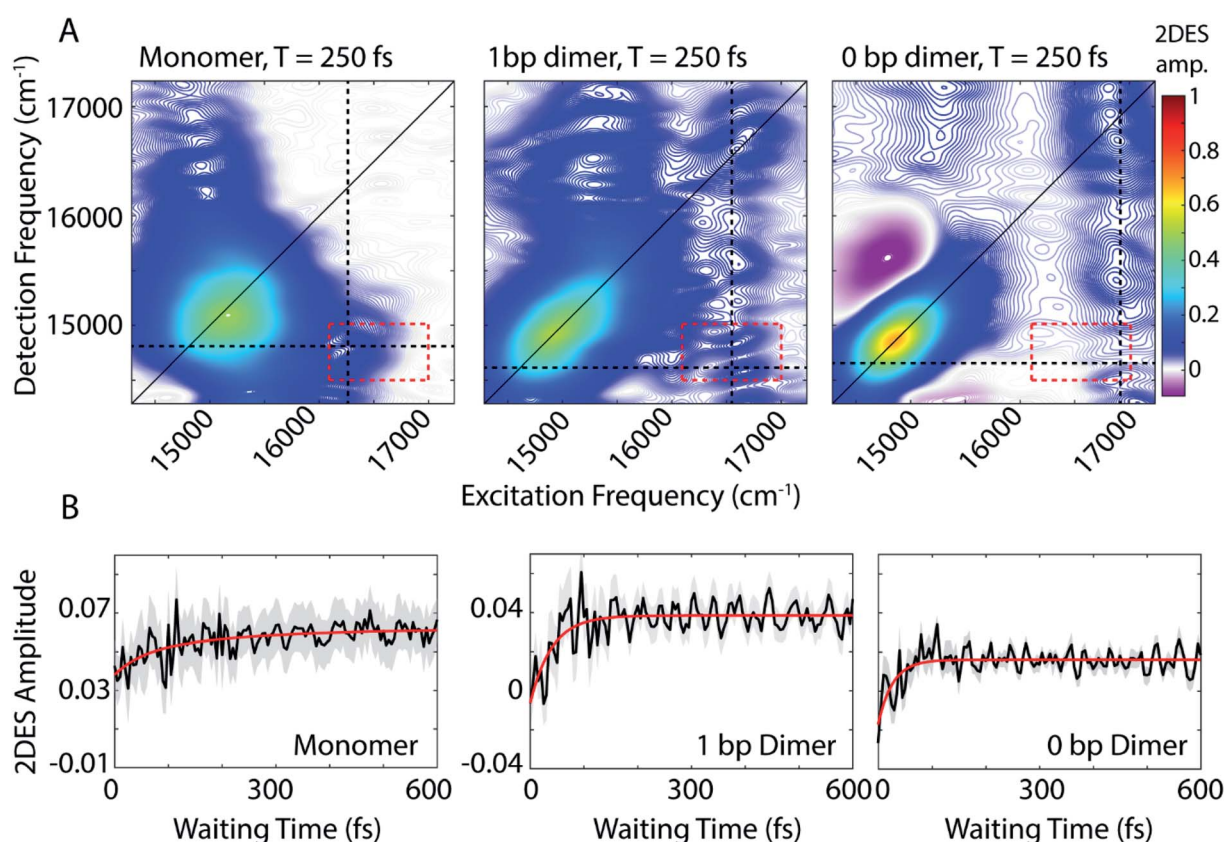
Fig. 2 (A) Absorptive 2DES spectra of monomer (left), 1 bp dimer (center), and 0 bp dimer (right) constructs at a waiting time of 250 fs. All presented spectra are the average of 16 individual data runs. The black dashed lines indicate the approximate spectral location of the 0–0 transition in detection frequency and 0–1 transition in excitation frequency. All points contained within the dashed red box are used to generate the power spectra in Fig. 4(B) 2DES signal as a function of waiting time ( T ) from the below diagonal cross peak location at the intersection of the dashed lines in (A). Monoexponential fits to the time traces are shown in red. Shaded gray region shows the standard error of the mean for the 16 data runs averaged to produce the mean waiting time trace (black).
